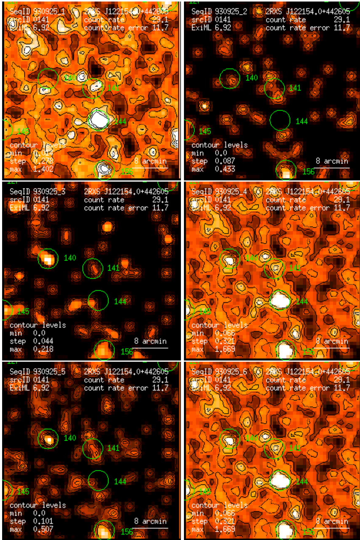
Figure 141: RASS 930925: detection 0141: band rate images, Gaussian filter: (1) PSPC channels 11 – 41, (2) 52 – 90, (3) 91 – 201, (4) 11 – 235, (5) 52 – 201, (6) 11 – 201. Broad band rates in counts/ks. Band rate contour levels in counts/ks/arcmin 2 .
