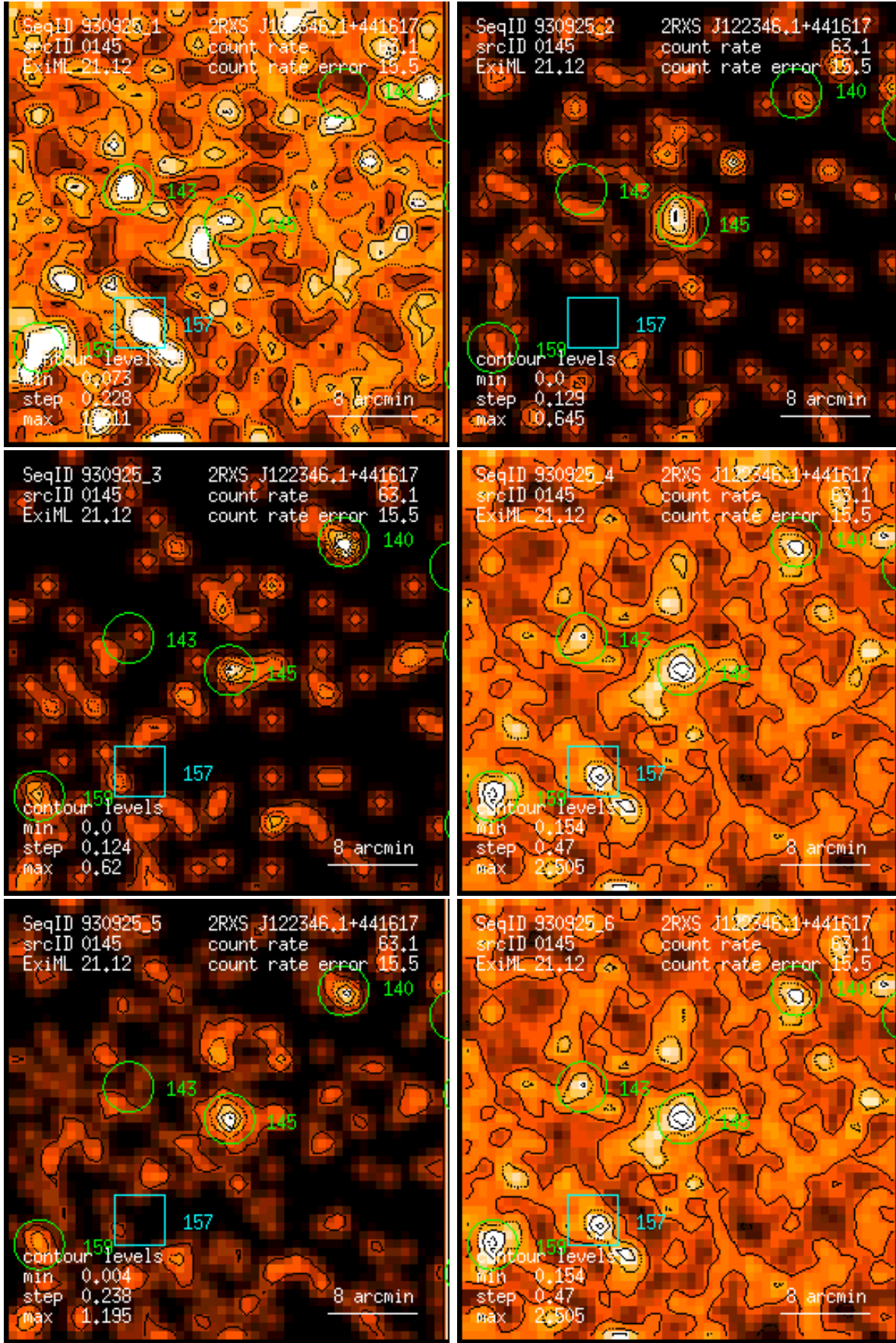
Figure 145: RASS 930925: detection 0145: band rate images, Gaussian filter: (1) PSPC channels 11 – 41, (2) 52 – 90, (3) 91 – 201, (4) 11 – 235, (5) 52 – 201, (6) 11 – 201. Broad band rates in counts/ks. Band rate contour levels in counts/ks/arcmin 2 .
