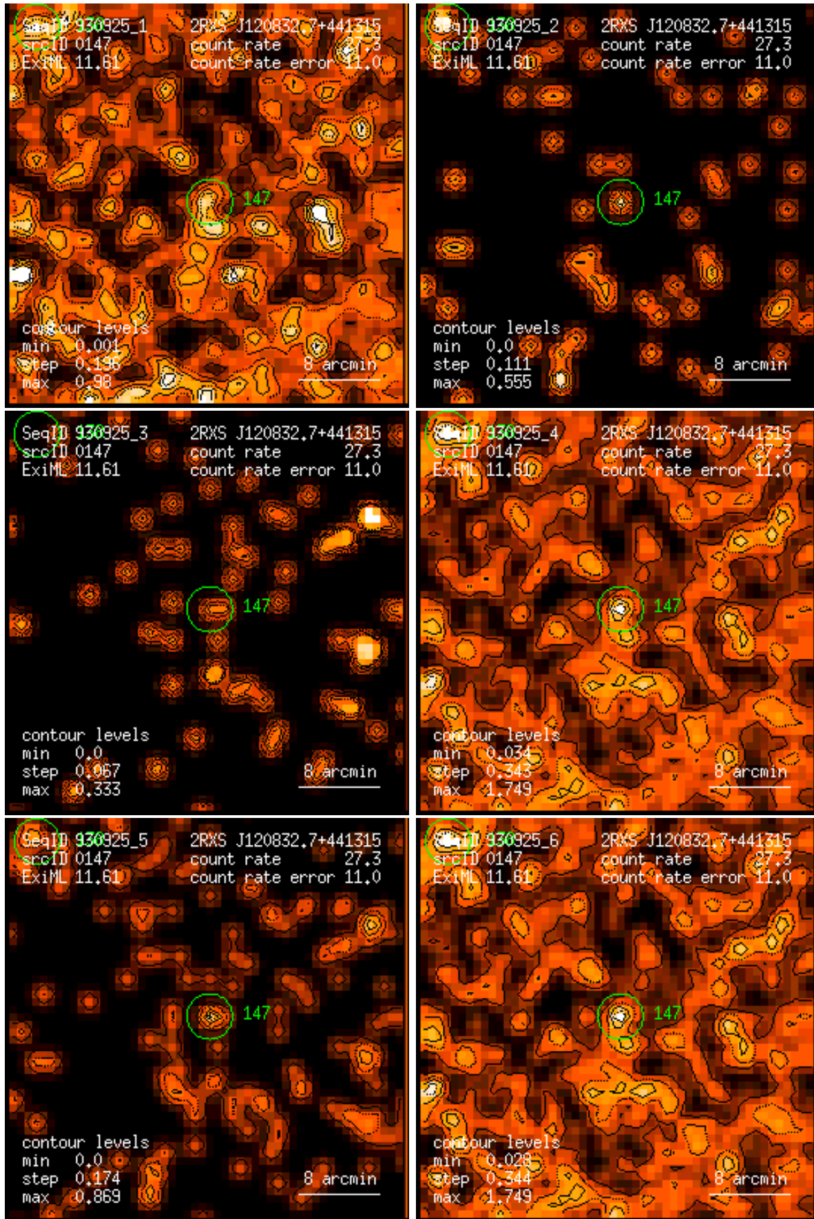
Figure 147: RASS 930925: detection 0147: band rate images, Gaussian filter: (1) PSPC channels 11 – 41, (2) 52 – 90, (3) 91 – 201, (4) 11 – 235, (5) 52 – 201, (6) 11 – 201. Broad band rates in counts/ks. Band rate contour levels in counts/ks/arcmin 2 .
