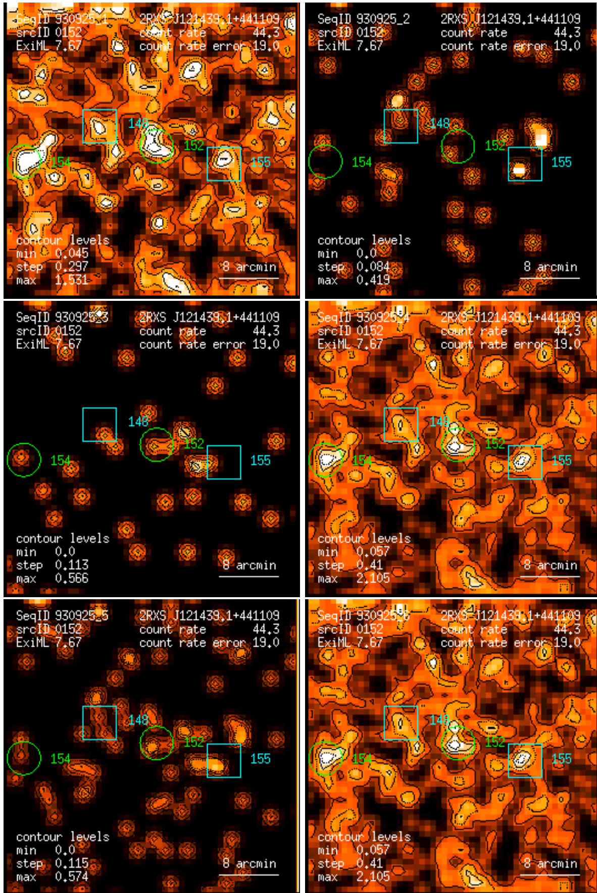
Figure 152: RASS 930925: detection 0152: band rate images, Gaussian filter: (1) PSPC channels 11 – 41, (2) 52 – 90, (3) 91 – 201, (4) 11 – 235, (5) 52 – 201, (6) 11 – 201. Broad band rates in counts/ks. Band rate contour levels in counts/ks/arcmin 2 .
