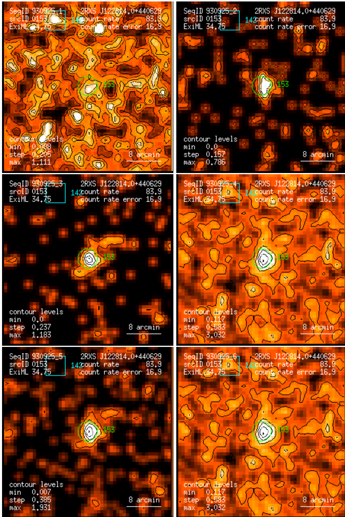
Figure 153: RASS 930925: detection 0153: band rate images, Gaussian filter: (1) PSPC channels 11 – 41, (2) 52 – 90, (3) 91 – 201, (4) 11 – 235, (5) 52 – 201, (6) 11 – 201. Broad band rates in counts/ks. Band rate contour levels in counts/ks/arcmin 2 .
