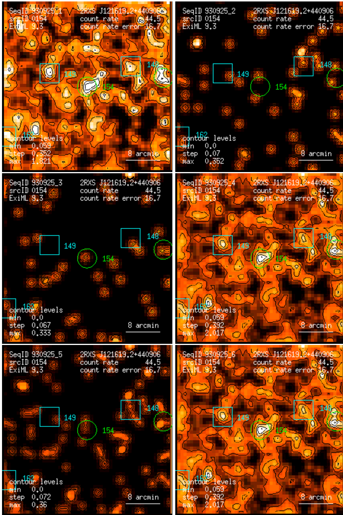
Figure 154: RASS 930925: detection 0154: band rate images, Gaussian filter: (1) PSPC channels 11 – 41, (2) 52 – 90, (3) 91 – 201, (4) 11 – 235, (5) 52 – 201, (6) 11 – 201. Broad band rates in counts/ks. Band rate contour levels in counts/ks/arcmin 2 .
