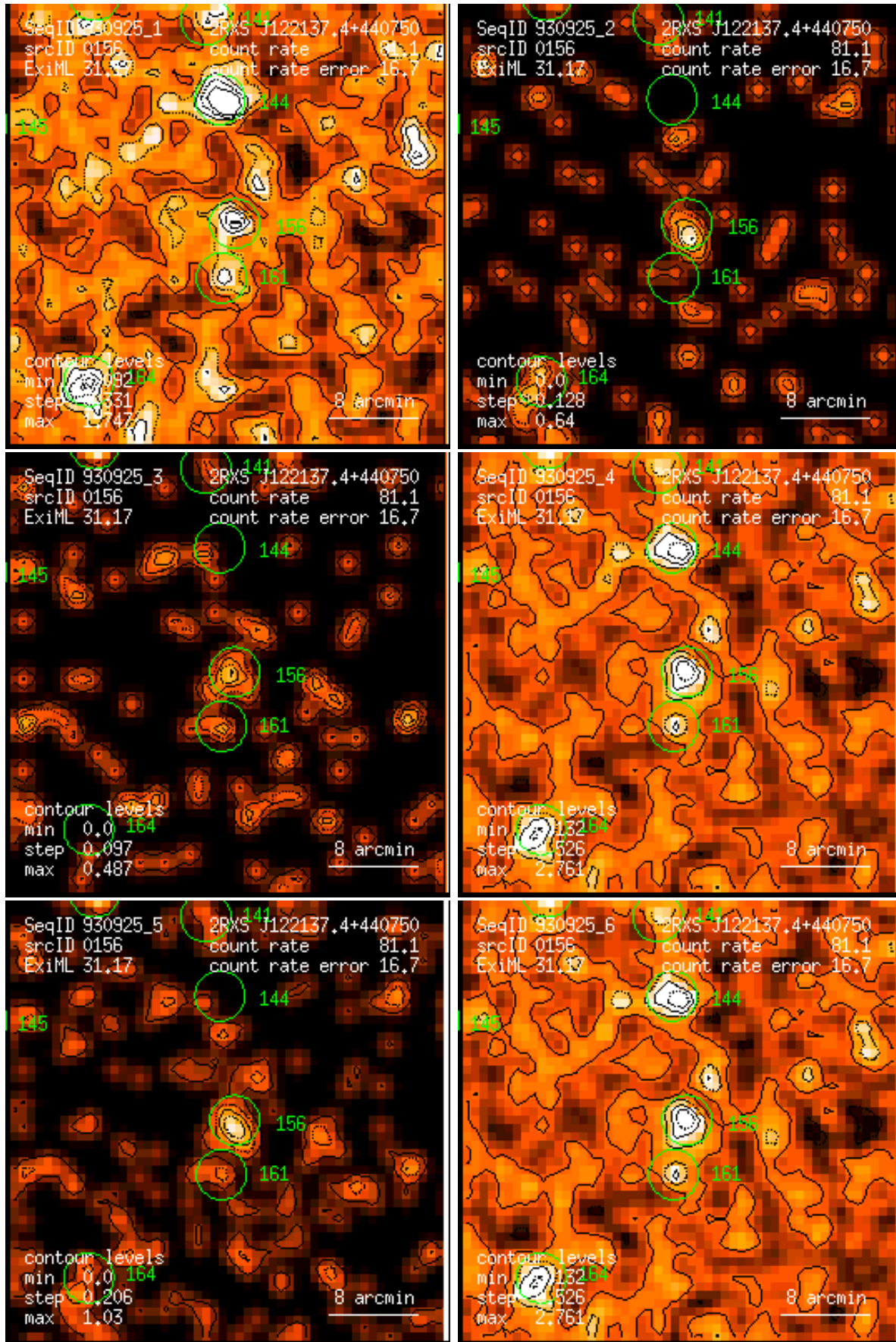
Figure 156: RASS 930925: detection 0156: band rate images, Gaussian filter: (1) PSPC channels 11 – 41, (2) 52 – 90, (3) 91 – 201, (4) 11 – 235, (5) 52 – 201, (6) 11 – 201. Broad band rates in counts/ks. Band rate contour levels in counts/ks/arcmin 2 .
