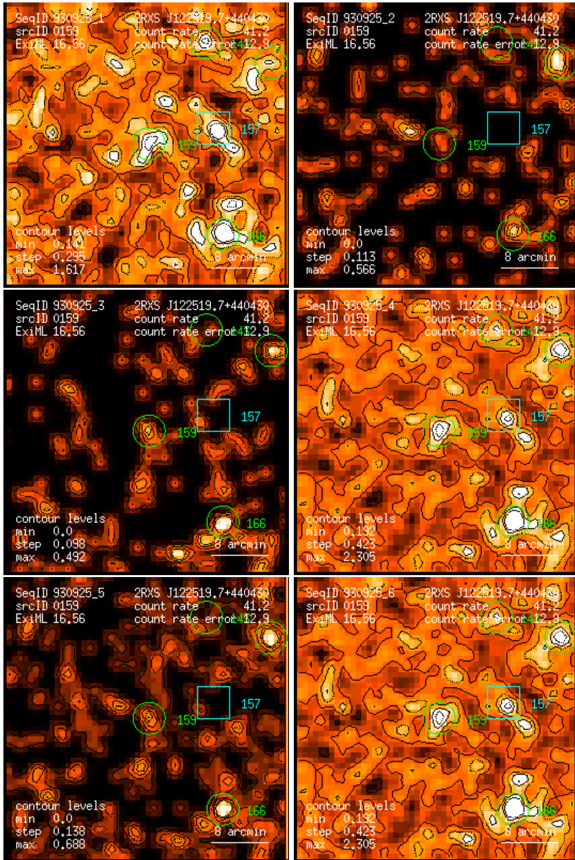
Figure 159: RASS 930925: detection 0159: band rate images, Gaussian filter: (1) PSPC channels 11 – 41, (2) 52 – 90, (3) 91 – 201, (4) 11 – 235, (5) 52 – 201, (6) 11 – 201. Broad band rates in counts/ks. Band rate contour levels in counts/ks/arcmin 2 .
