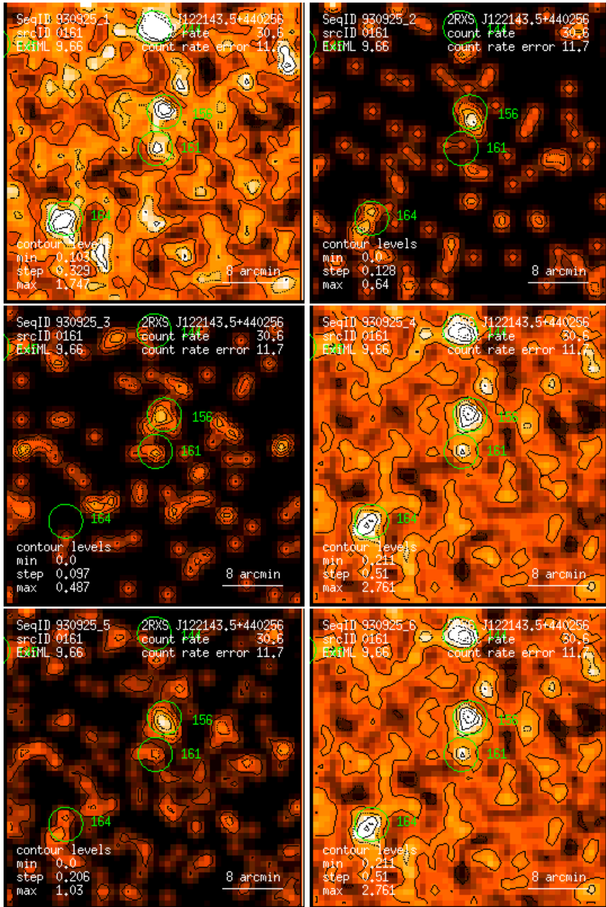
Figure 161: RASS 930925: detection 0161: band rate images, Gaussian filter: (1) PSPC channels 11 – 41, (2) 52 – 90, (3) 91 – 201, (4) 11 – 235, (5) 52 – 201, (6) 11 – 201. Broad band rates in counts/ks. Band rate contour levels in counts/ks/arcmin 2 .
