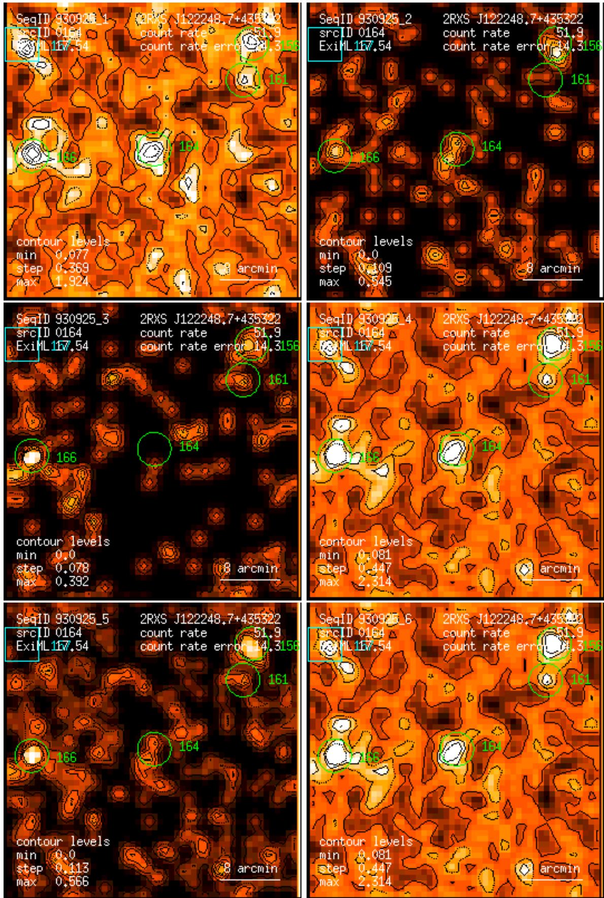
Figure 164: RASS 930925: detection 0164: band rate images, Gaussian filter: (1) PSPC channels 11 – 41, (2) 52 – 90, (3) 91 – 201, (4) 11 – 235, (5) 52 – 201, (6) 11 – 201. Broad band rates in counts/ks. Band rate contour levels in counts/ks/arcmin 2 .
