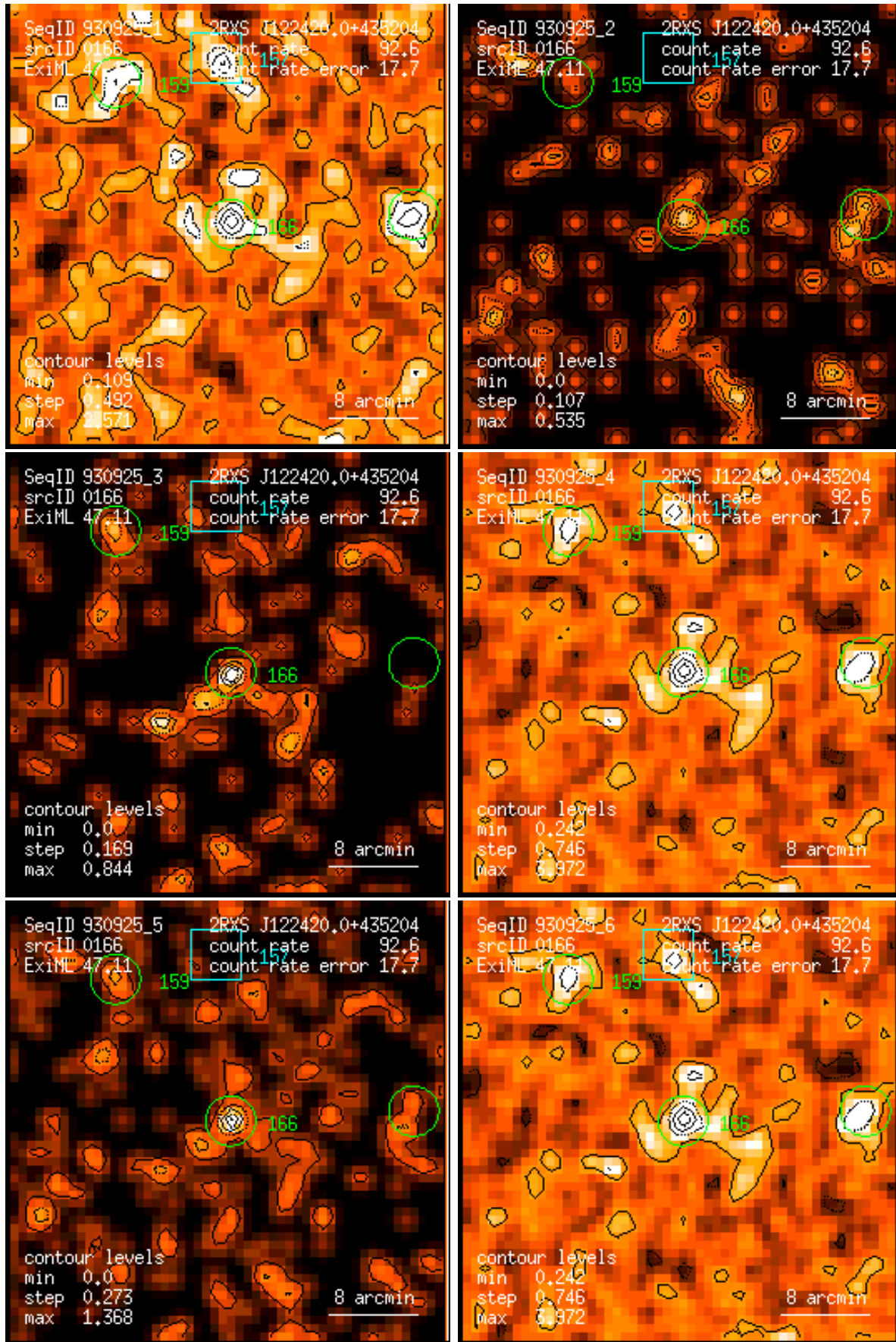
Figure 166: RASS 930925: detection 0166: band rate images, Gaussian filter: (1) PSPC channels 11 – 41, (2) 52 – 90, (3) 91 – 201, (4) 11 – 235, (5) 52 – 201, (6) 11 – 201. Broad band rates in counts/ks. Band rate contour levels in counts/ks/arcmin 2 .
