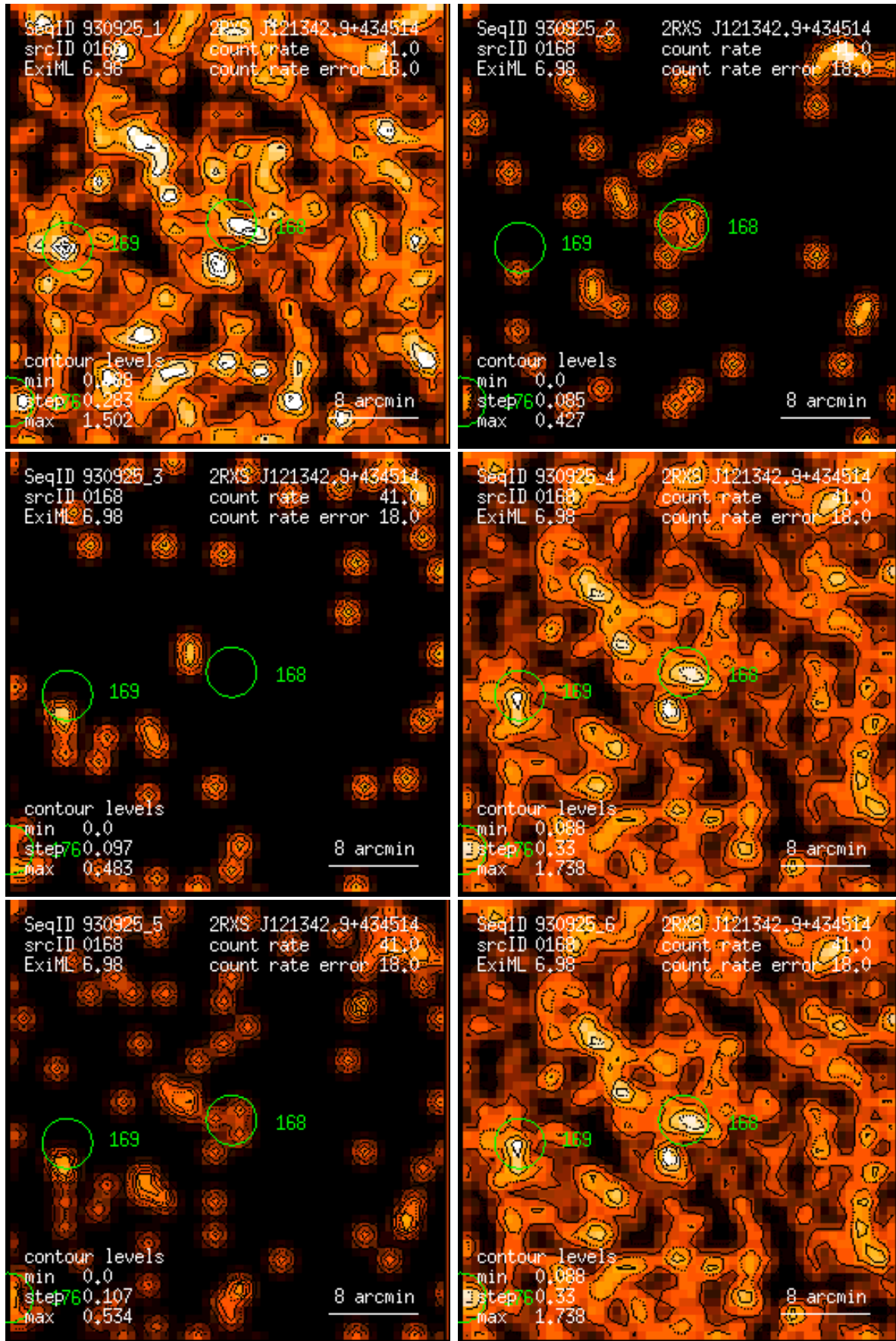
Figure 168: RASS 930925: detection 0168: band rate images, Gaussian filter: (1) PSPC channels 11 – 41, (2) 52 – 90, (3) 91 – 201, (4) 11 – 235, (5) 52 – 201, (6) 11 – 201. Broad band rates in counts/ks. Band rate contour levels in counts/ks/arcmin 2 .
