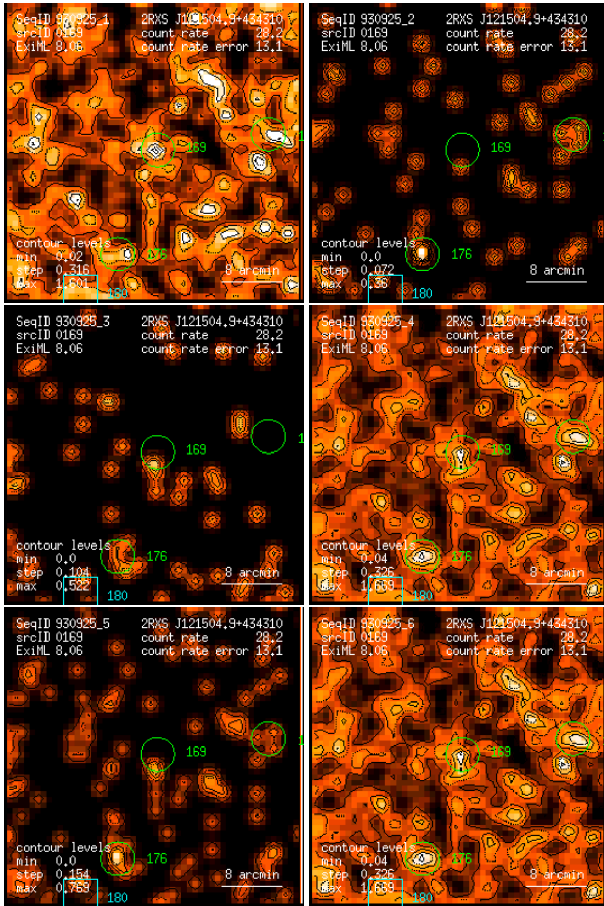
Figure 169: RASS 930925: detection 0169: band rate images, Gaussian filter: (1) PSPC channels 11 – 41, (2) 52 – 90, (3) 91 – 201, (4) 11 – 235, (5) 52 – 201, (6) 11 – 201. Broad band rates in counts/ks. Band rate contour levels in counts/ks/arcmin 2 .
