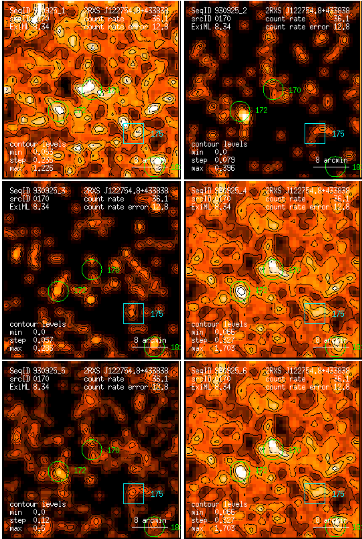
Figure 170: RASS 930925: detection 0170: band rate images, Gaussian filter: (1) PSPC channels 11 – 41, (2) 52 – 90, (3) 91 – 201, (4) 11 – 235, (5) 52 – 201, (6) 11 – 201. Broad band rates in counts/ks. Band rate contour levels in counts/ks/arcmin 2 .
