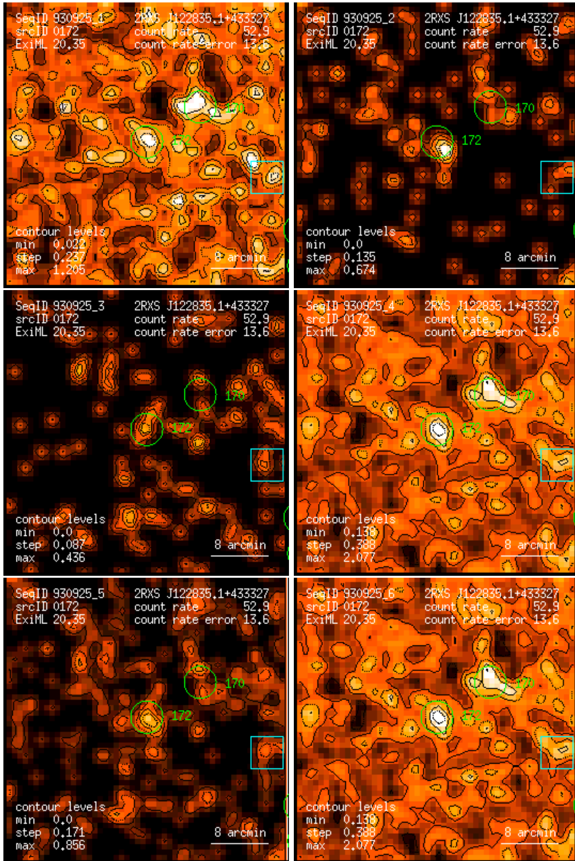
Figure 172: RASS 930925: detection 0172: band rate images, Gaussian filter: (1) PSPC channels 11 – 41, (2) 52 – 90, (3) 91 – 201, (4) 11 – 235, (5) 52 – 201, (6) 11 – 201. Broad band rates in counts/ks. Band rate contour levels in counts/ks/arcmin 2 .
