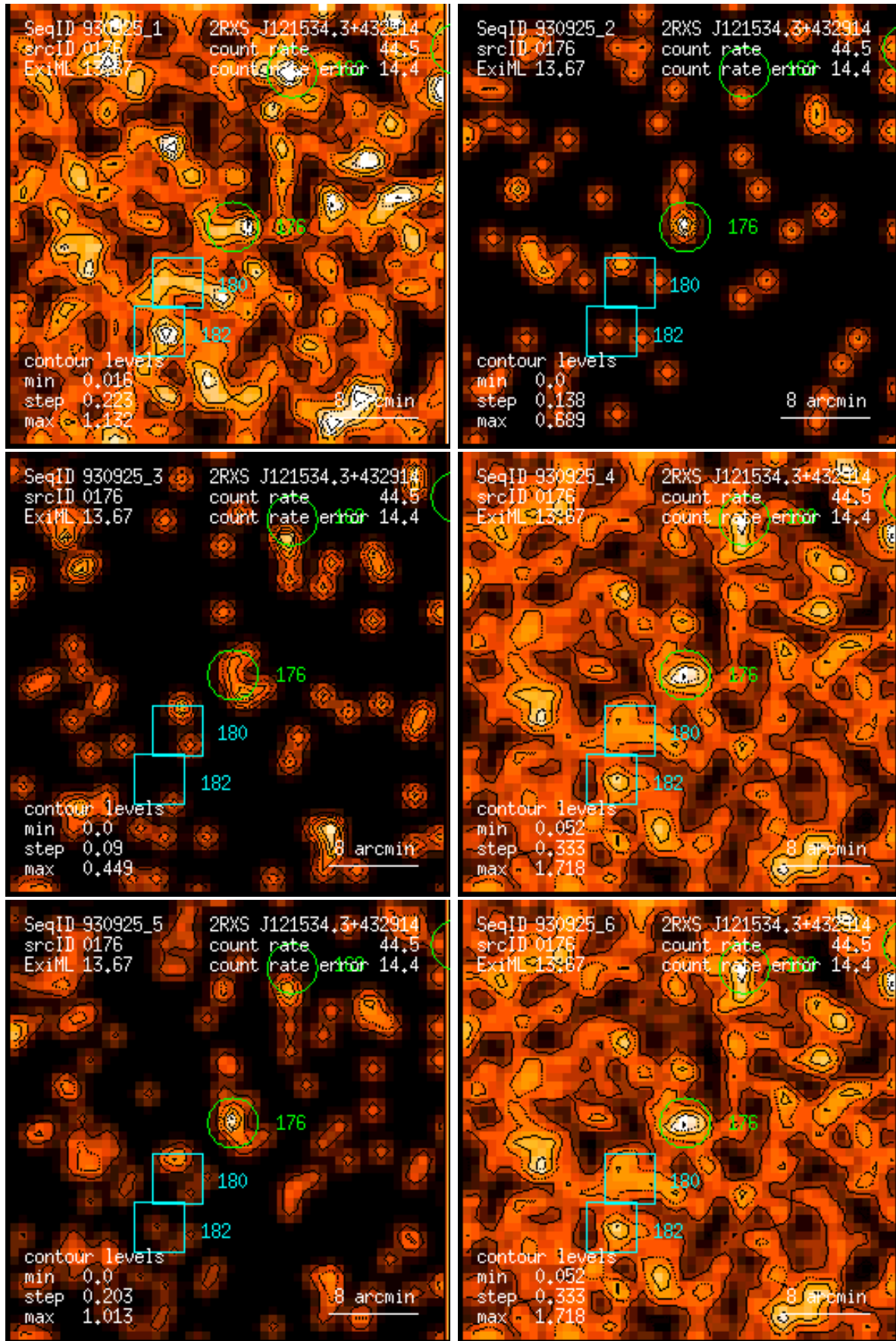
Figure 176: RASS 930925: detection 0176: band rate images, Gaussian filter: (1) PSPC channels 11 – 41, (2) 52 – 90, (3) 91 – 201, (4) 11 – 235, (5) 52 – 201, (6) 11 – 201. Broad band rates in counts/ks. Band rate contour levels in counts/ks/arcmin 2 .
