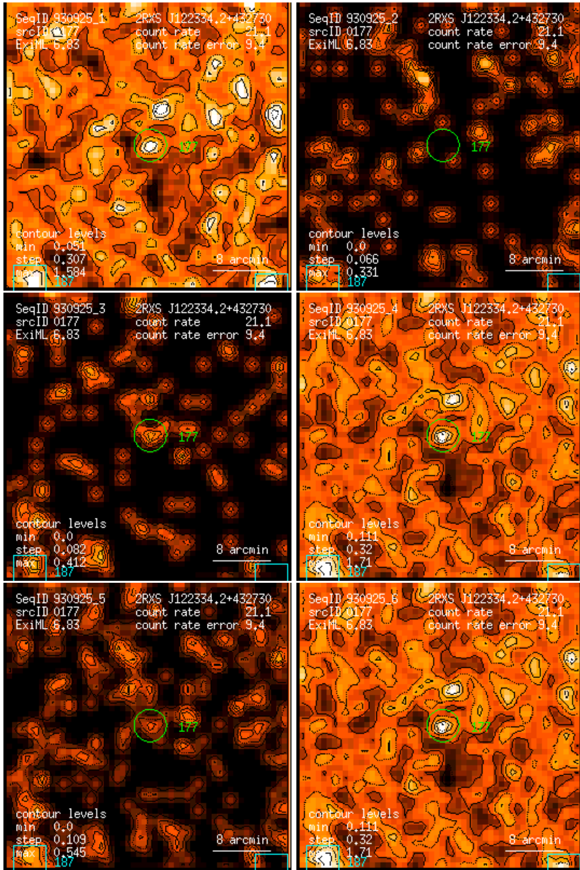
Figure 177: RASS 930925: detection 0177: band rate images, Gaussian filter: (1) PSPC channels 11 – 41, (2) 52 – 90, (3) 91 – 201, (4) 11 – 235, (5) 52 – 201, (6) 11 – 201. Broad band rates in counts/ks. Band rate contour levels in counts/ks/arcmin 2 .
