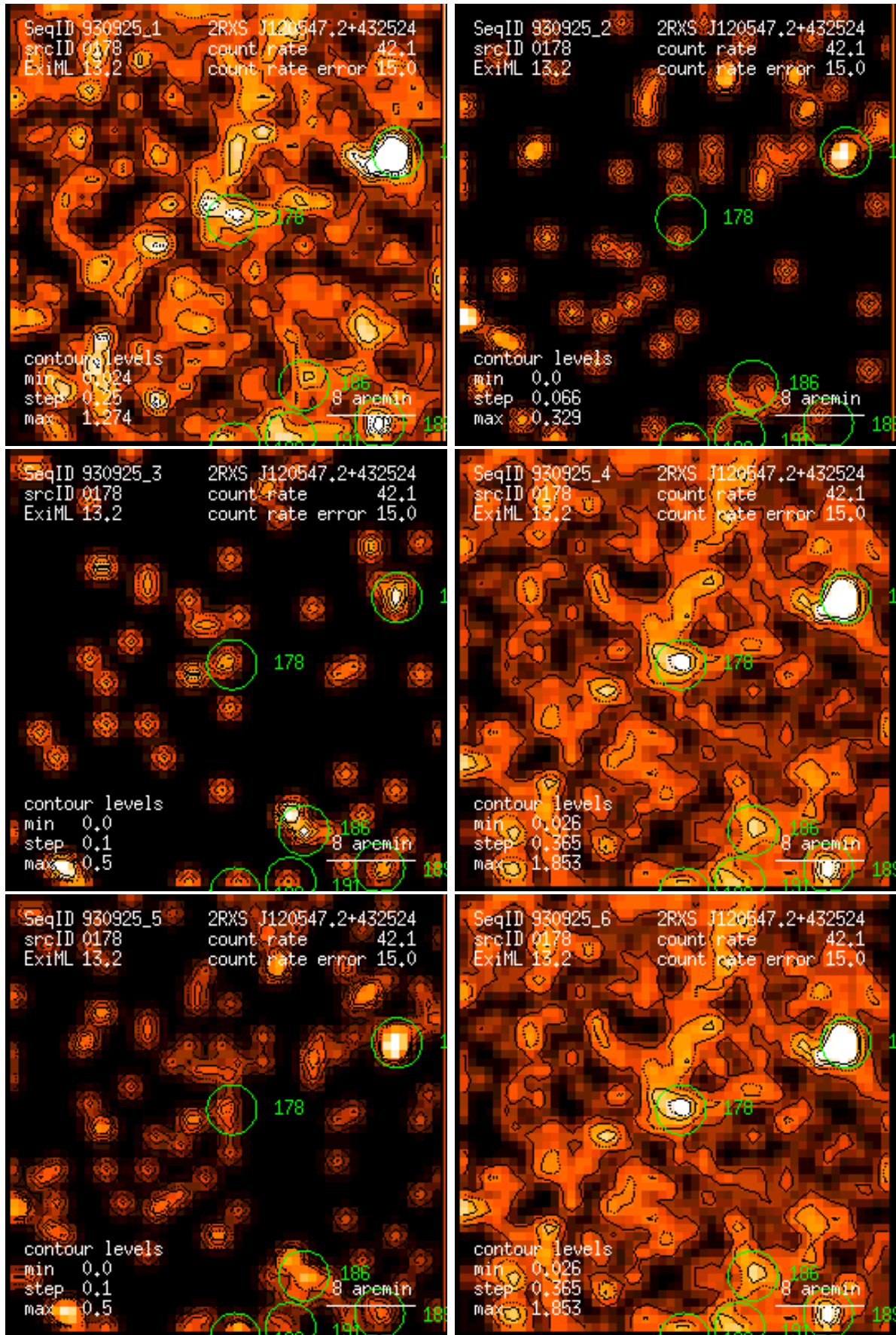
Figure 178: RASS 930925: detection 0178: band rate images, Gaussian filter: (1) PSPC channels 11 – 41, (2) 52 – 90, (3) 91 – 201, (4) 11 – 235, (5) 52 – 201, (6) 11 – 201. Broad band rates in counts/ks. Band rate contour levels in counts/ks/arcmin 2 .
