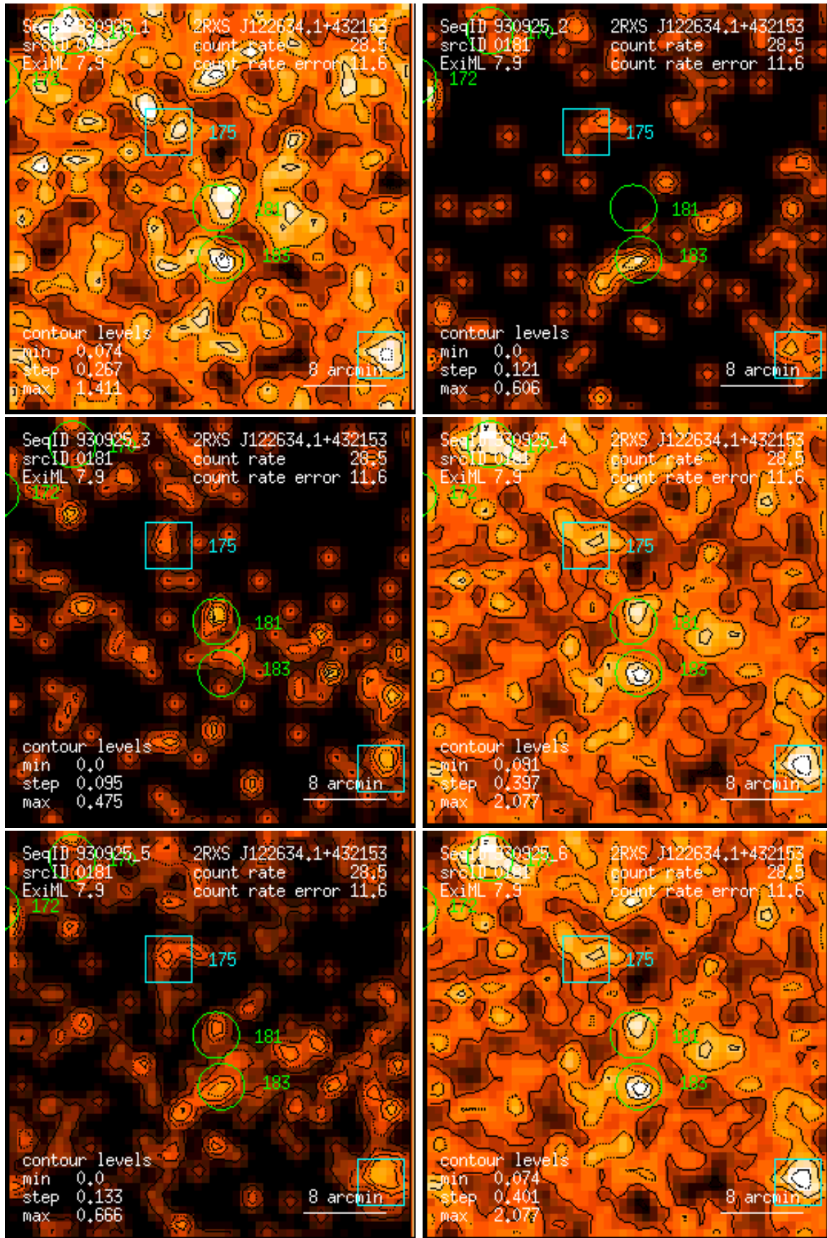
Figure 181: RASS 930925: detection 0181: band rate images, Gaussian filter: (1) PSPC channels 11 – 41, (2) 52 – 90, (3) 91 – 201, (4) 11 – 235, (5) 52 – 201, (6) 11 – 201. Broad band rates in counts/ks. Band rate contour levels in counts/ks/arcmin 2 .
