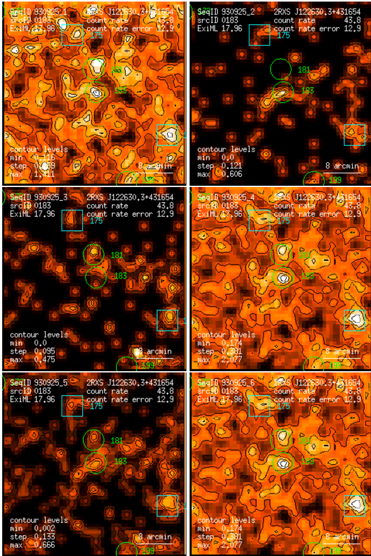
Figure 183: RASS 930925: detection 0183: band rate images, Gaussian filter: (1) PSPC channels 11 – 41, (2) 52 – 90, (3) 91 – 201, (4) 11 – 235, (5) 52 – 201, (6) 11 – 201. Broad band rates in counts/ks. Band rate contour levels in counts/ks/arcmin 2 .
