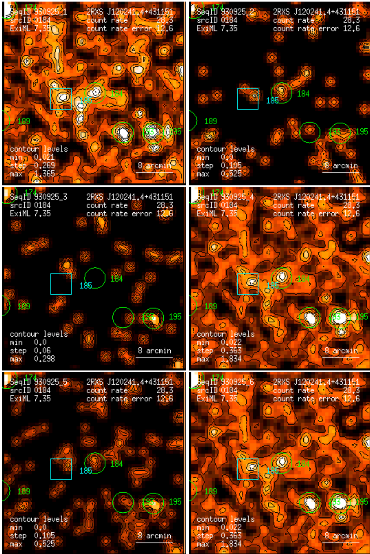
Figure 184: RASS 930925: detection 0184: band rate images, Gaussian filter: (1) PSPC channels 11 – 41, (2) 52 – 90, (3) 91 – 201, (4) 11 – 235, (5) 52 – 201, (6) 11 – 201. Broad band rates in counts/ks. Band rate contour levels in counts/ks/arcmin 2 .
