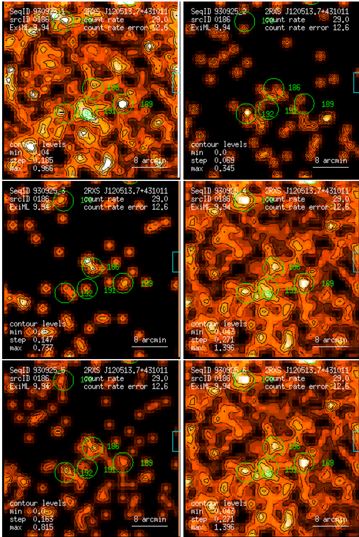
Figure 186: RASS 930925: detection 0186: band rate images, Gaussian filter: (1) PSPC channels 11 – 41, (2) 52 – 90, (3) 91 – 201, (4) 11 – 235, (5) 52 – 201, (6) 11 – 201. Broad band rates in counts/ks. Band rate contour levels in counts/ks/arcmin 2 .
