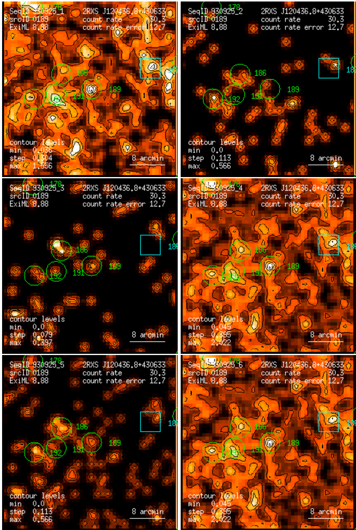
Figure 189: RASS 930925: detection 0189: band rate images, Gaussian filter: (1) PSPC channels 11 – 41, (2) 52 – 90, (3) 91 – 201, (4) 11 – 235, (5) 52 – 201, (6) 11 – 201. Broad band rates in counts/ks. Band rate contour levels in counts/ks/arcmin 2 .
