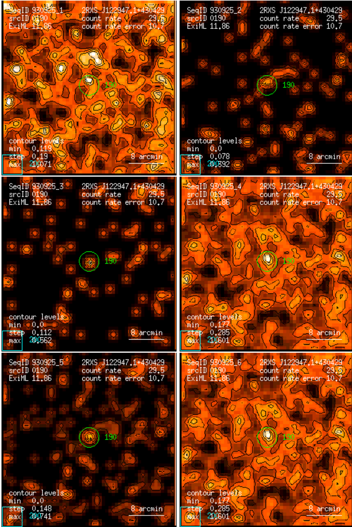
Figure 190: RASS 930925: detection 0190: band rate images, Gaussian filter: (1) PSPC channels 11 – 41, (2) 52 – 90, (3) 91 – 201, (4) 11 – 235, (5) 52 – 201, (6) 11 – 201. Broad band rates in counts/ks. Band rate contour levels in counts/ks/arcmin 2 .
