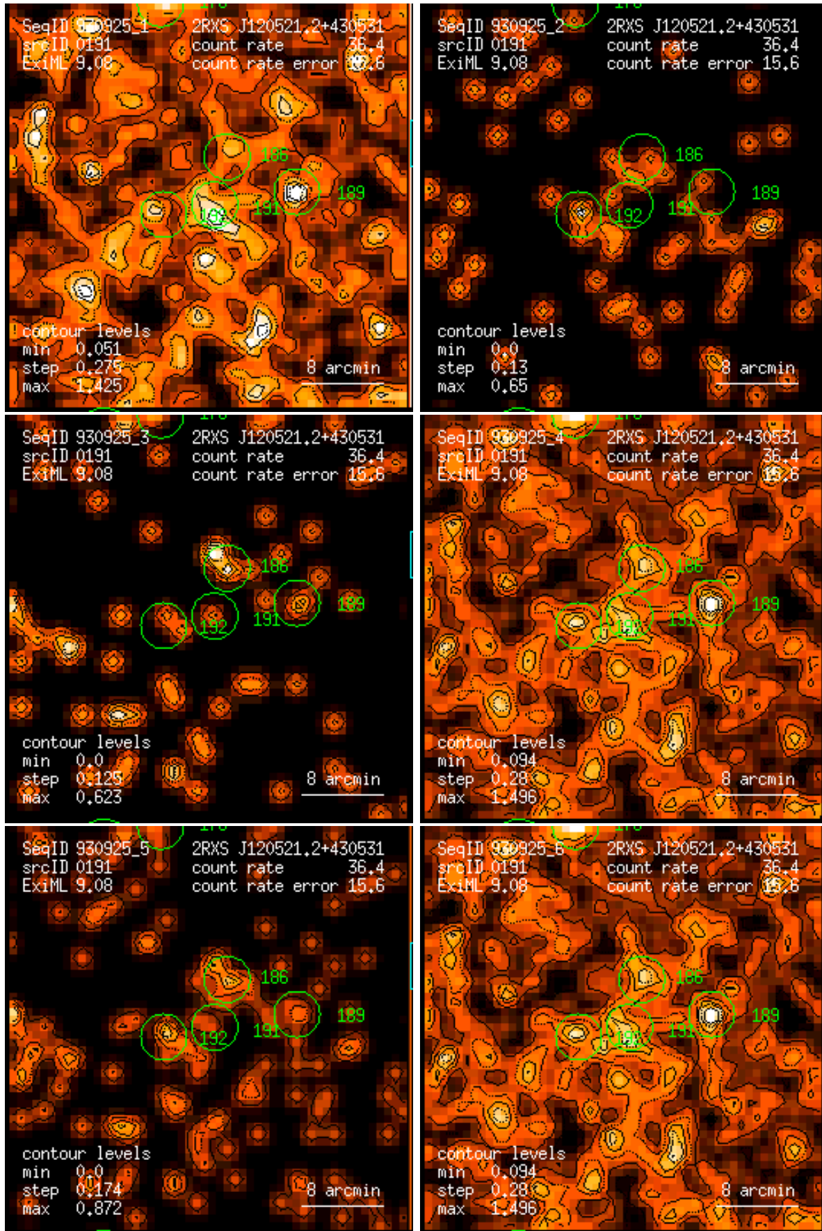
Figure 191: RASS 930925: detection 0191: band rate images, Gaussian filter: (1) PSPC channels 11 – 41, (2) 52 – 90, (3) 91 – 201, (4) 11 – 235, (5) 52 – 201, (6) 11 – 201. Broad band rates in counts/ks. Band rate contour levels in counts/ks/arcmin 2 .
