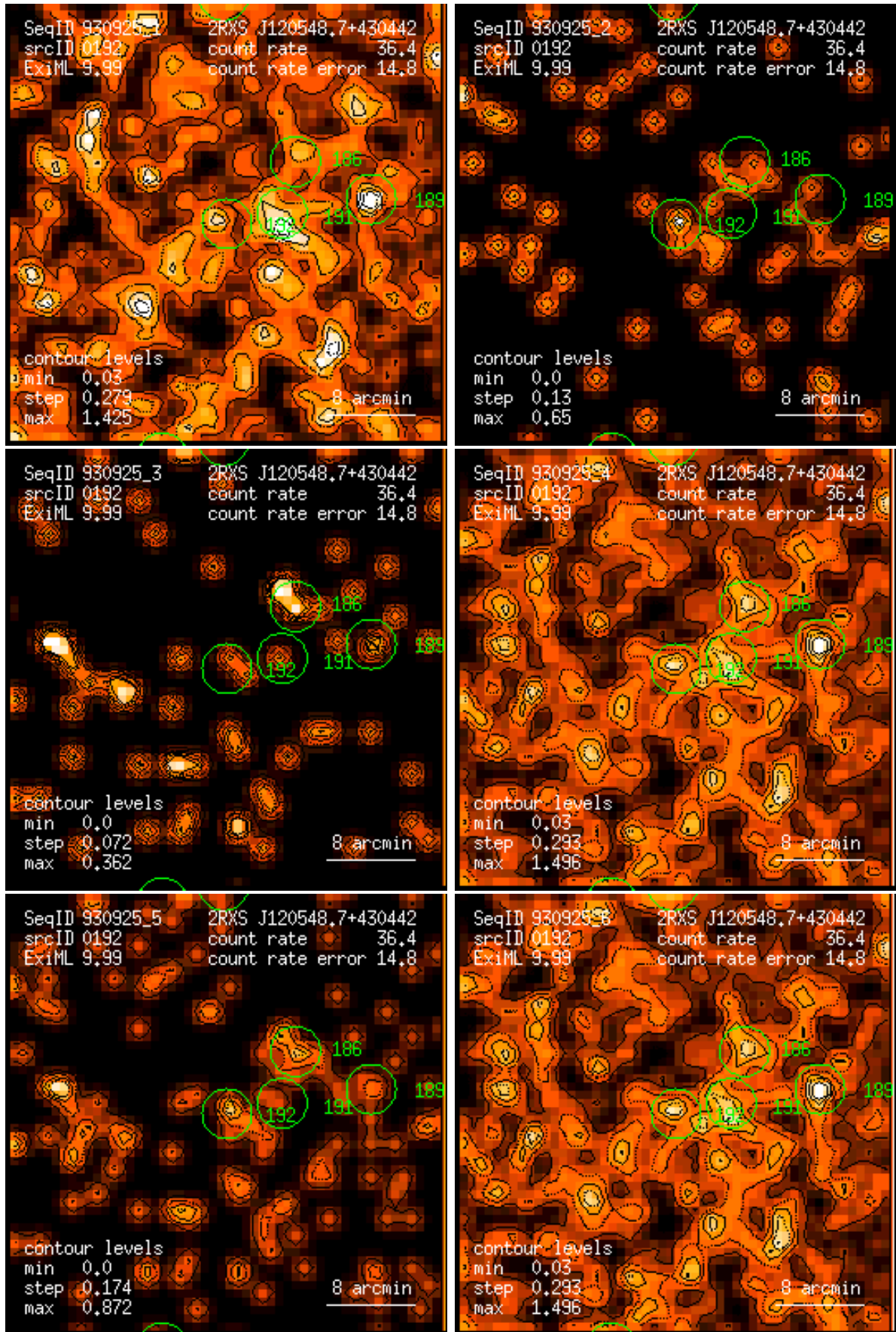
Figure 192: RASS 930925: detection 0192: band rate images, Gaussian filter: (1) PSPC channels 11 – 41, (2) 52 – 90, (3) 91 – 201, (4) 11 – 235, (5) 52 – 201, (6) 11 – 201. Broad band rates in counts/ks. Band rate contour levels in counts/ks/arcmin 2 .
