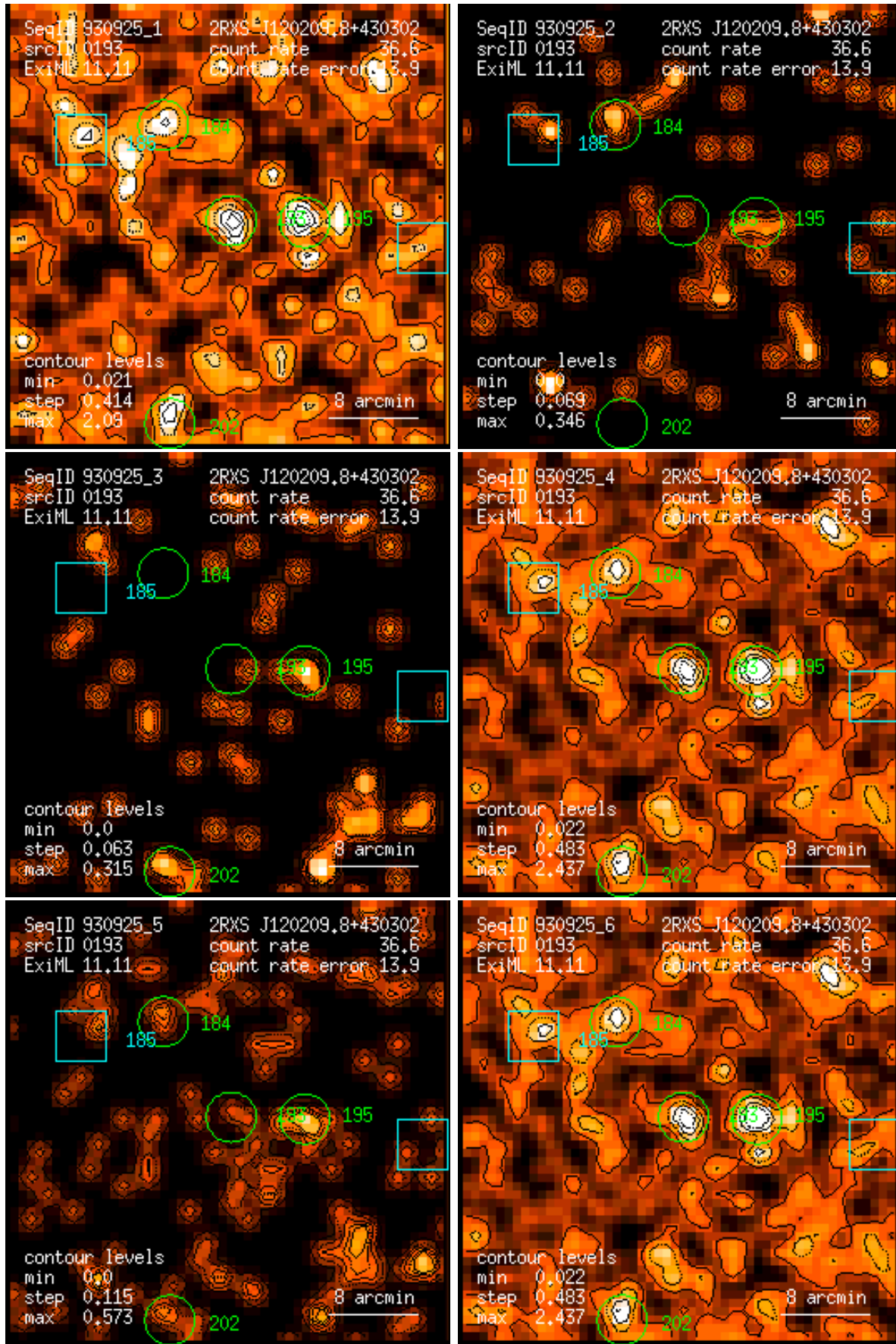
Figure 193: RASS 930925: detection 0193: band rate images, Gaussian filter: (1) PSPC channels 11 – 41, (2) 52 – 90, (3) 91 – 201, (4) 11 – 235, (5) 52 – 201, (6) 11 – 201. Broad band rates in counts/ks. Band rate contour levels in counts/ks/arcmin 2 .
