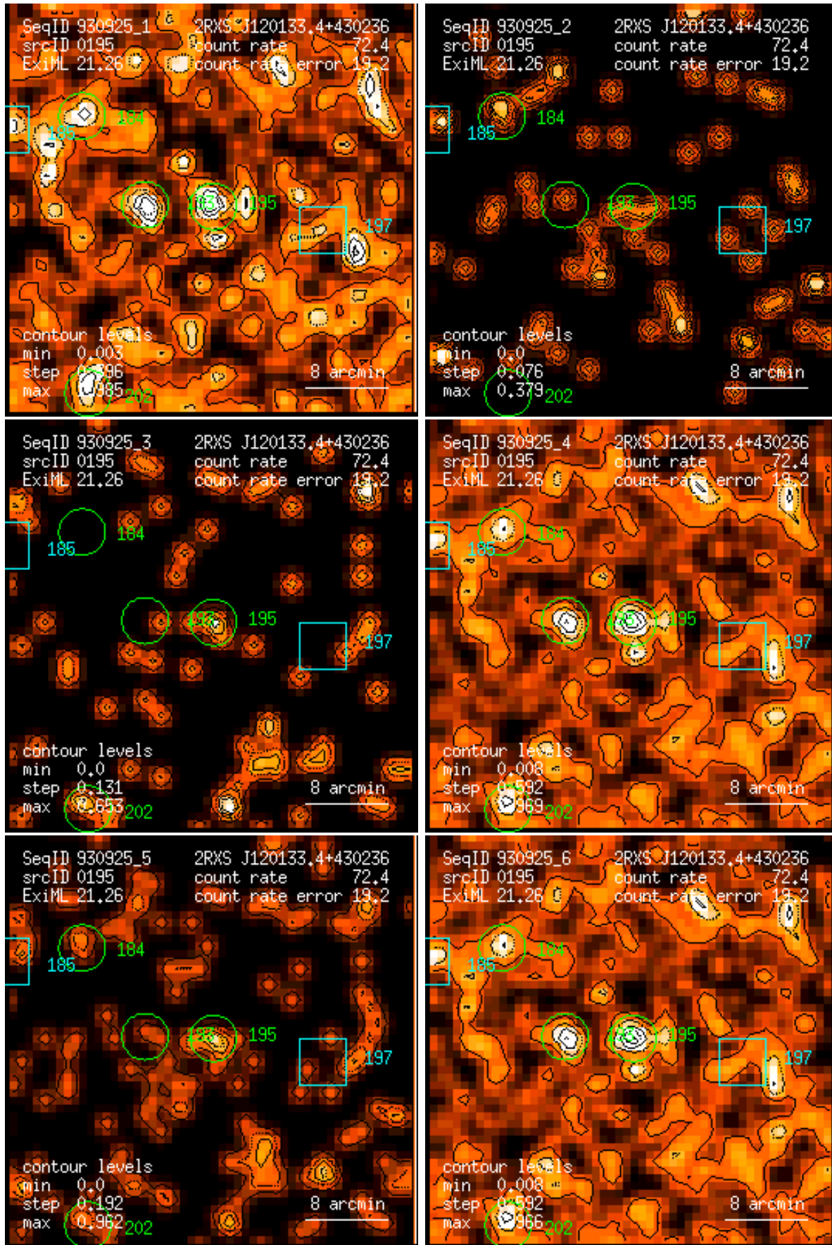
Figure 195: RASS 930925: detection 0195: band rate images, Gaussian filter: (1) PSPC channels 11 – 41, (2) 52 – 90, (3) 91 – 201, (4) 11 – 235, (5) 52 – 201, (6) 11 – 201. Broad band rates in counts/ks. Band rate contour levels in counts/ks/arcmin 2 .
