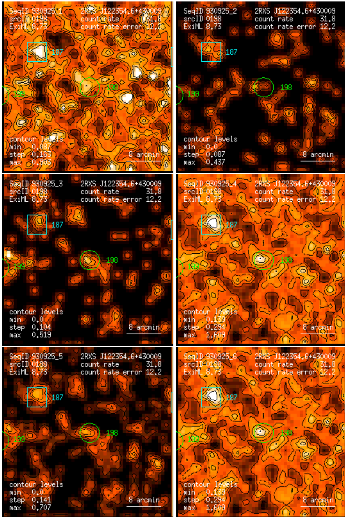
Figure 198: RASS 930925: detection 0198: band rate images, Gaussian filter: (1) PSPC channels 11 – 41, (2) 52 – 90, (3) 91 – 201, (4) 11 – 235, (5) 52 – 201, (6) 11 – 201. Broad band rates in counts/ks. Band rate contour levels in counts/ks/arcmin 2 .
