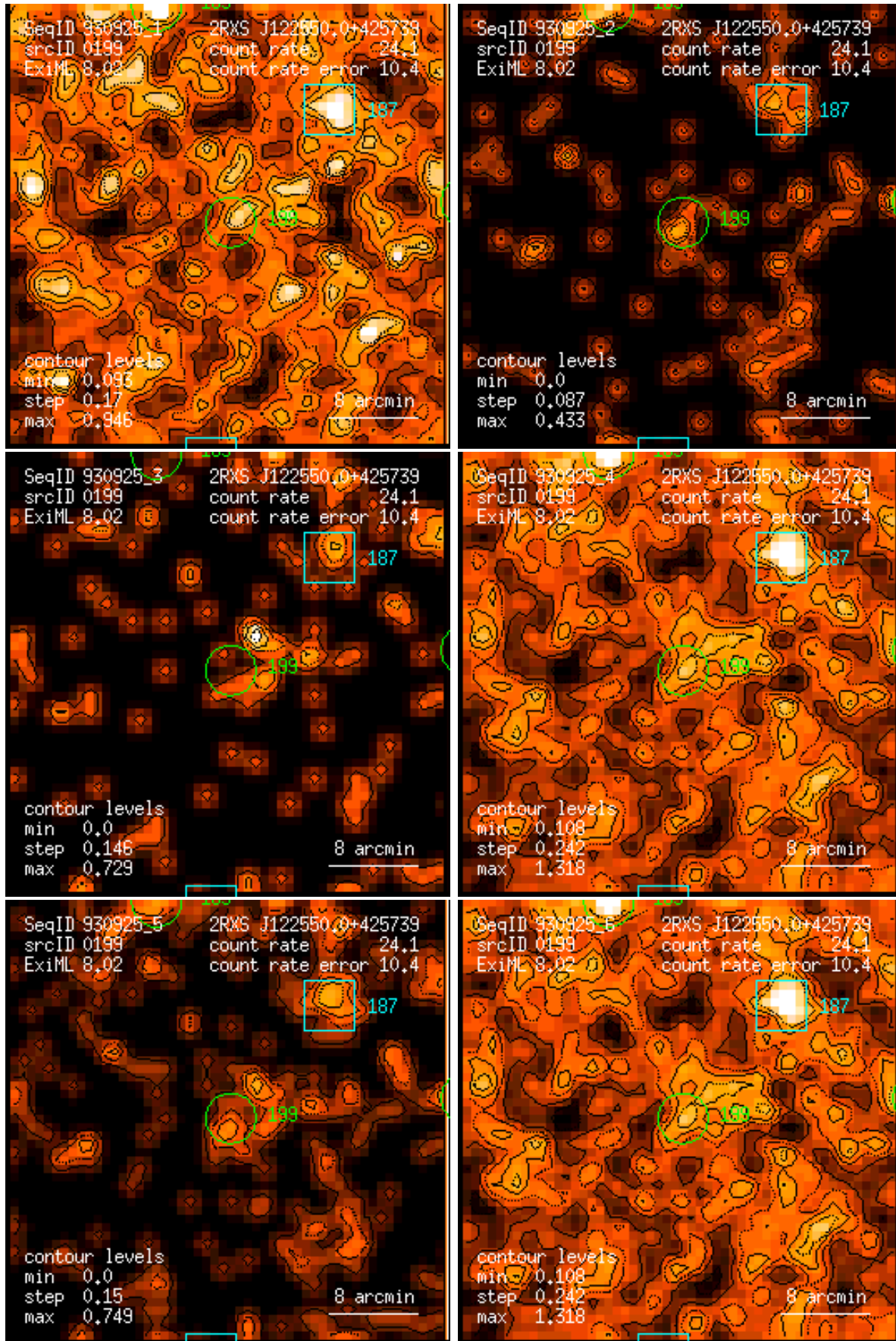
Figure 199: RASS 930925: detection 0199: band rate images, Gaussian filter: (1) PSPC channels 11 – 41, (2) 52 – 90, (3) 91 – 201, (4) 11 – 235, (5) 52 – 201, (6) 11 – 201. Broad band rates in counts/ks. Band rate contour levels in counts/ks/arcmin 2 .
