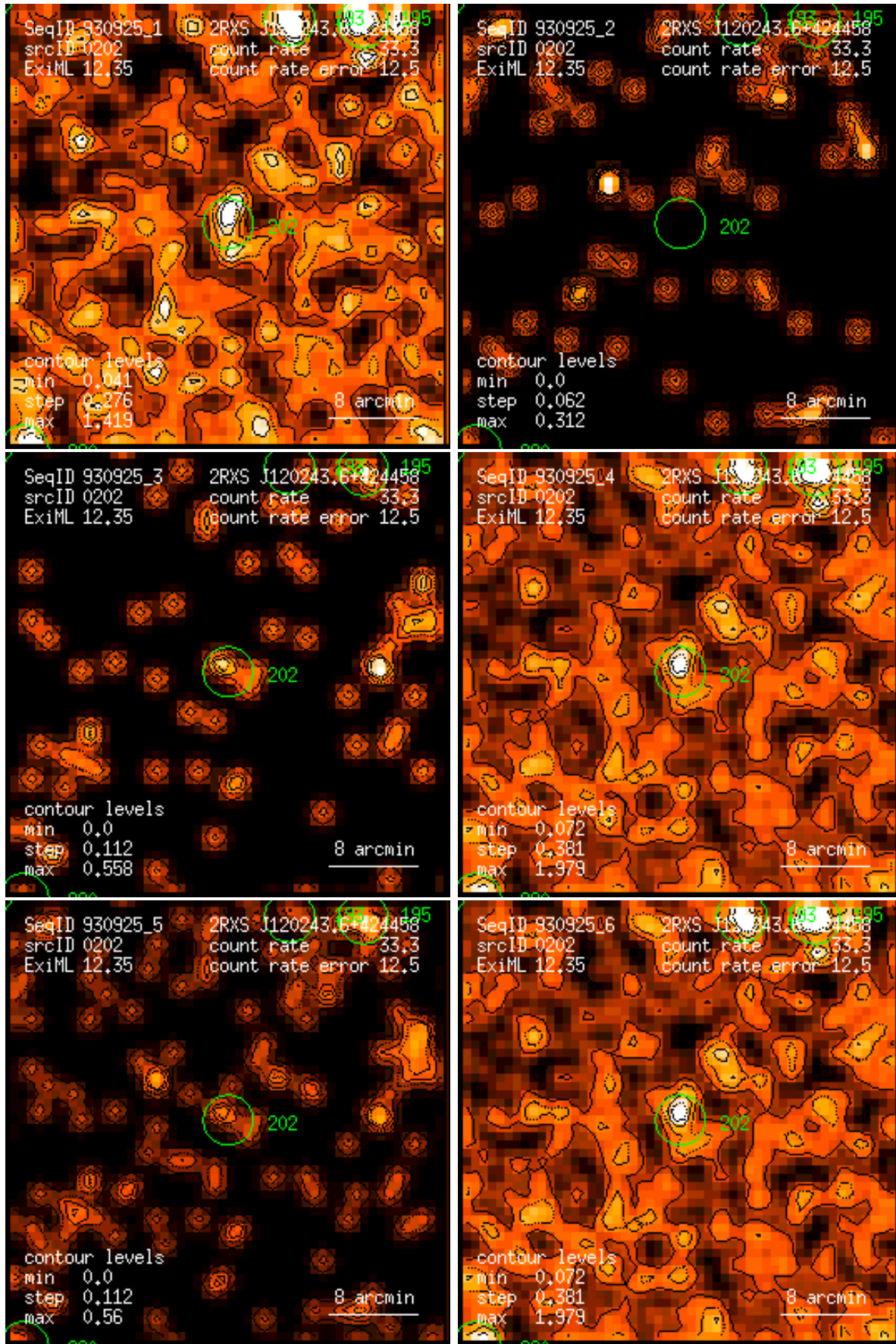
Figure 202: RASS 930925: detection 0202: band rate images, Gaussian filter: (1) PSPC channels 11 – 41, (2) 52 – 90, (3) 91 – 201, (4) 11 – 235, (5) 52 – 201, (6) 11 – 201. Broad band rates in counts/ks. Band rate contour levels in counts/ks/arcmin 2 .
