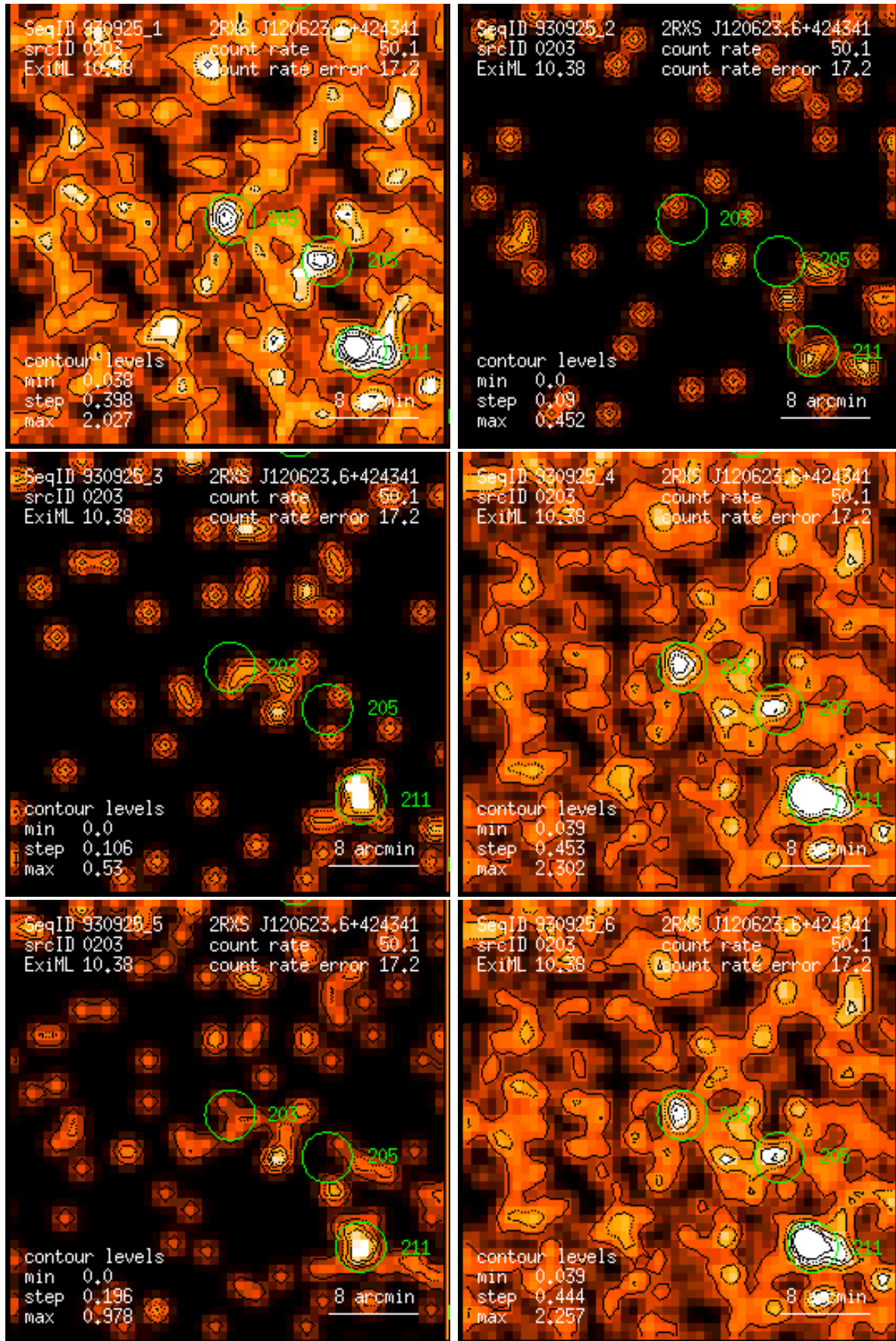
Figure 203: RASS 930925: detection 0203: band rate images, Gaussian filter: (1) PSPC channels 11 – 41, (2) 52 – 90, (3) 91 – 201, (4) 11 – 235, (5) 52 – 201, (6) 11 – 201. Broad band rates in counts/ks. Band rate contour levels in counts/ks/arcmin 2 .
