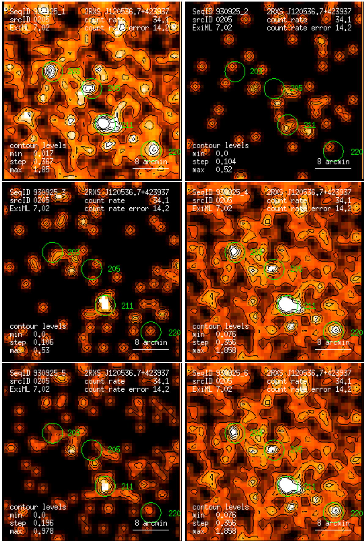
Figure 205: RASS 930925: detection 0205: band rate images, Gaussian filter: (1) PSPC channels 11 – 41, (2) 52 – 90, (3) 91 – 201, (4) 11 – 235, (5) 52 – 201, (6) 11 – 201. Broad band rates in counts/ks. Band rate contour levels in counts/ks/arcmin 2 .
