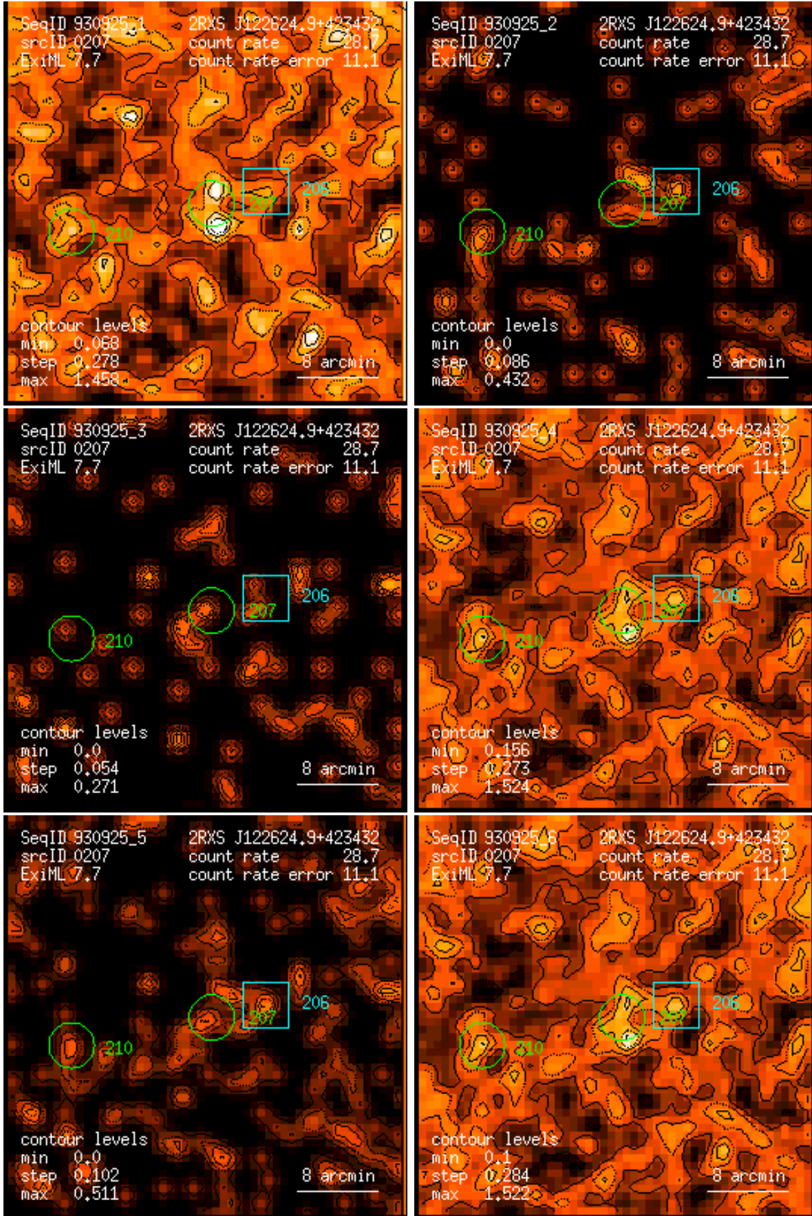
Figure 207: RASS 930925: detection 0207: band rate images, Gaussian filter: (1) PSPC channels 11 – 41, (2) 52 – 90, (3) 91 – 201, (4) 11 – 235, (5) 52 – 201, (6) 11 – 201. Broad band rates in counts/ks. Band rate contour levels in counts/ks/arcmin 2 .
