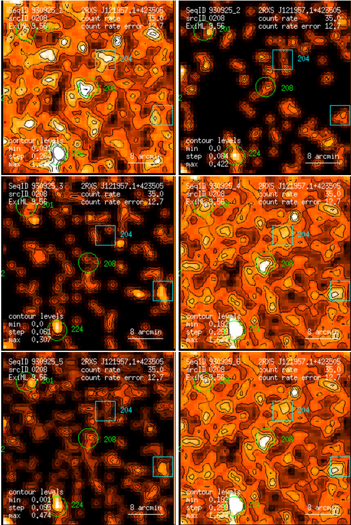
Figure 208: RASS 930925: detection 0208: band rate images, Gaussian filter: (1) PSPC channels 11 – 41, (2) 52 – 90, (3) 91 – 201, (4) 11 – 235, (5) 52 – 201, (6) 11 – 201. Broad band rates in counts/ks. Band rate contour levels in counts/ks/arcmin 2 .
