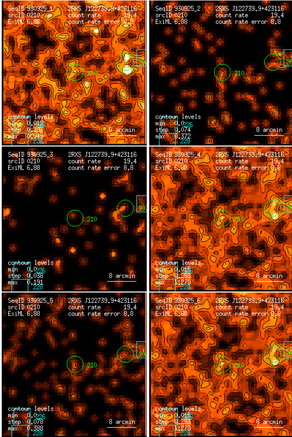
Figure 210: RASS 930925: detection 0210: band rate images, Gaussian filter: (1) PSPC channels 11 – 41, (2) 52 – 90, (3) 91 – 201, (4) 11 – 235, (5) 52 – 201, (6) 11 – 201. Broad band rates in counts/ks. Band rate contour levels in counts/ks/arcmin 2 .
