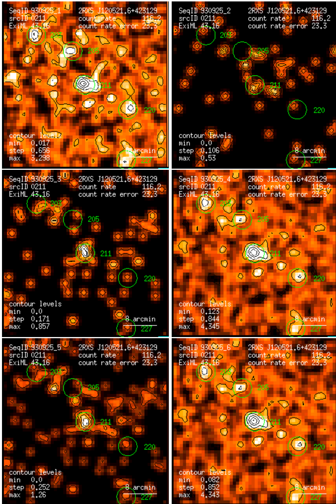
Figure 211: RASS 930925: detection 0211: band rate images, Gaussian filter: (1) PSPC channels 11 – 41, (2) 52 – 90, (3) 91 – 201, (4) 11 – 235, (5) 52 – 201, (6) 11 – 201. Broad band rates in counts/ks. Band rate contour levels in counts/ks/arcmin 2 .
