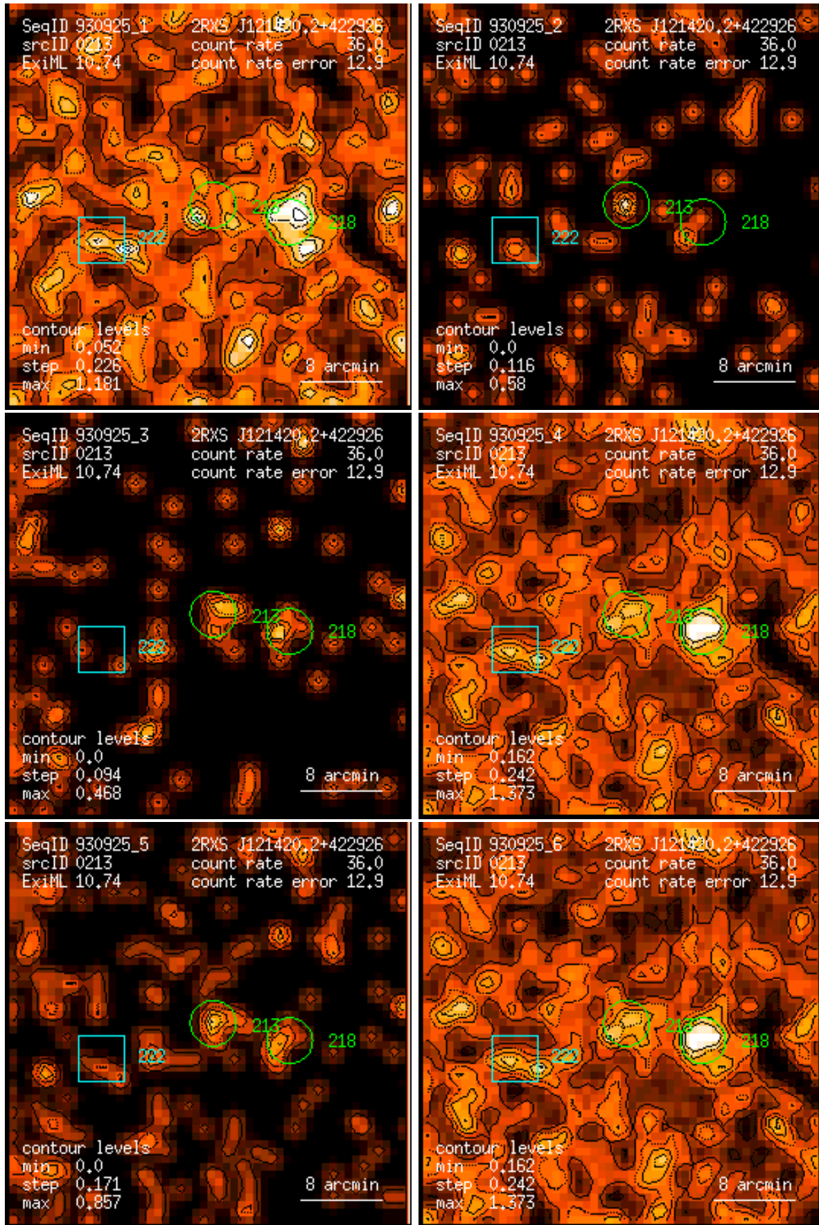
Figure 213: RASS 930925: detection 0213: band rate images, Gaussian filter: (1) PSPC channels 11 – 41, (2) 52 – 90, (3) 91 – 201, (4) 11 – 235, (5) 52 – 201, (6) 11 – 201. Broad band rates in counts/ks. Band rate contour levels in counts/ks/arcmin 2 .
