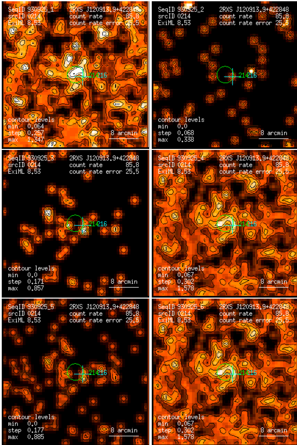
Figure 214: RASS 930925: detection 0214: band rate images, Gaussian filter: (1) PSPC channels 11 – 41, (2) 52 – 90, (3) 91 – 201, (4) 11 – 235, (5) 52 – 201, (6) 11 – 201. Broad band rates in counts/ks. Band rate contour levels in counts/ks/arcmin 2 .
