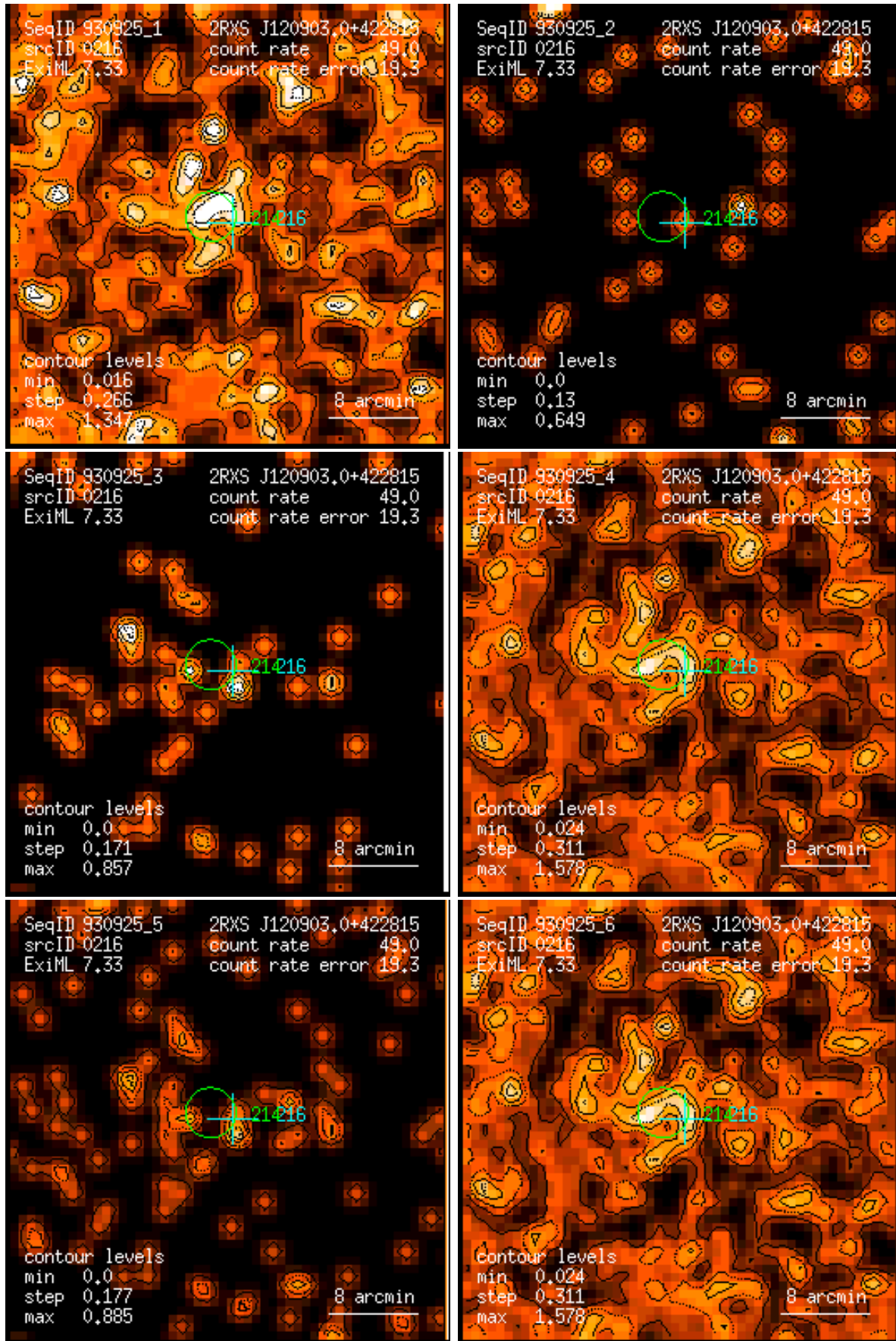
Figure 216: RASS 930925: detection 0216: band rate images, Gaussian filter: (1) PSPC channels 11 – 41, (2) 52 – 90, (3) 91 – 201, (4) 11 – 235, (5) 52 – 201, (6) 11 – 201. Broad band rates in counts/ks. Band rate contour levels in counts/ks/arcmin 2 .
