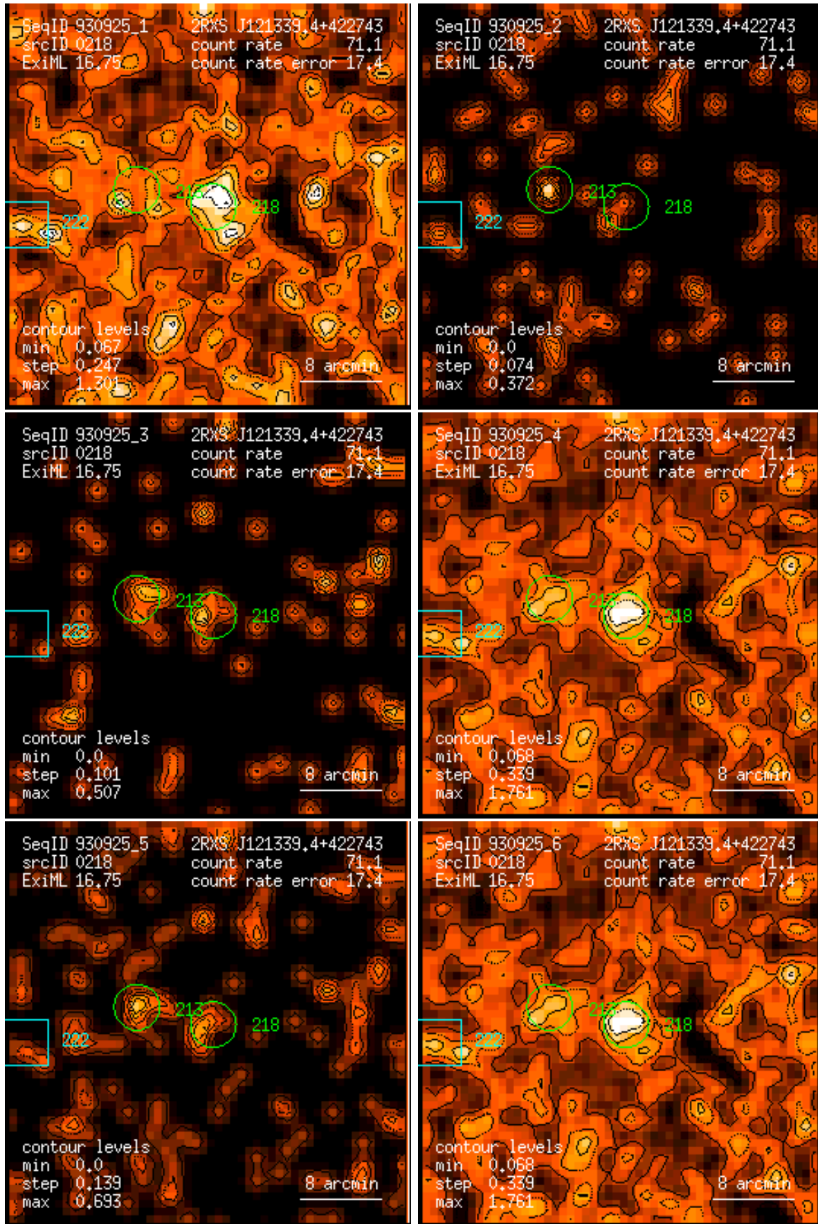
Figure 218: RASS 930925: detection 0218: band rate images, Gaussian filter: (1) PSPC channels 11 – 41, (2) 52 – 90, (3) 91 – 201, (4) 11 – 235, (5) 52 – 201, (6) 11 – 201. Broad band rates in counts/ks. Band rate contour levels in counts/ks/arcmin 2 .
