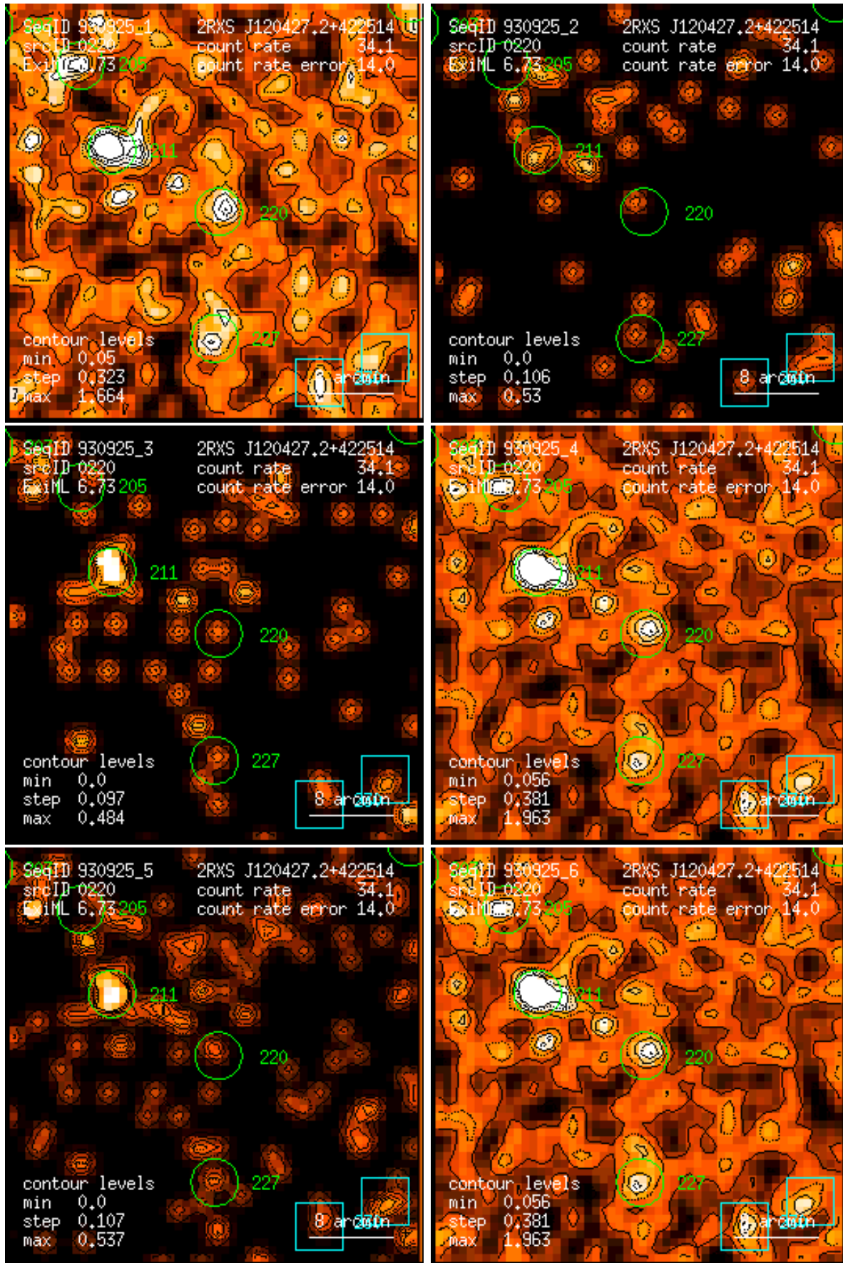
Figure 220: RASS 930925: detection 0220: band rate images, Gaussian filter: (1) PSPC channels 11 – 41, (2) 52 – 90, (3) 91 – 201, (4) 11 – 235, (5) 52 – 201, (6) 11 – 201. Broad band rates in counts/ks. Band rate contour levels in counts/ks/arcmin 2 .
