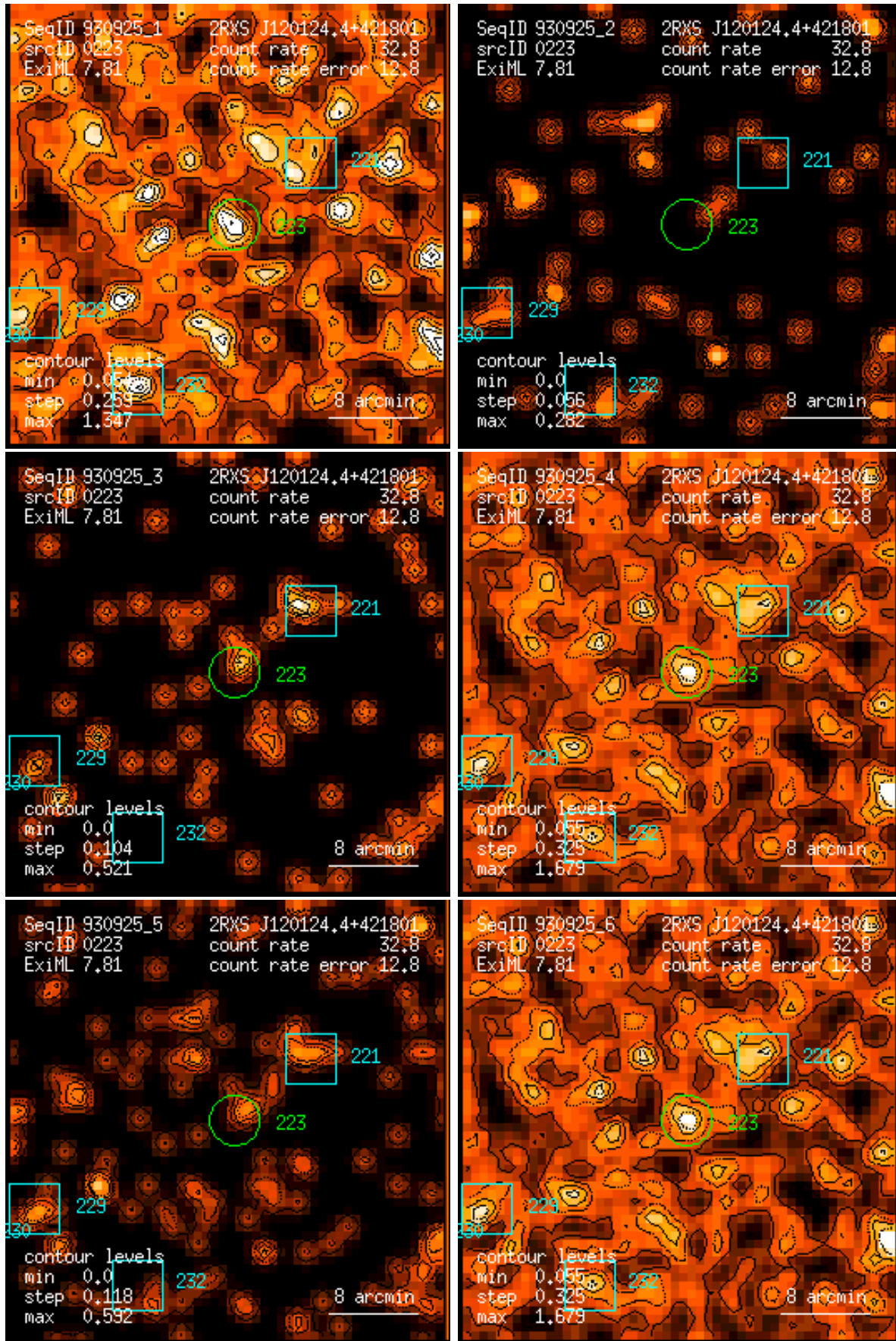
Figure 223: RASS 930925: detection 0223: band rate images, Gaussian filter: (1) PSPC channels 11 – 41, (2) 52 – 90, (3) 91 – 201, (4) 11 – 235, (5) 52 – 201, (6) 11 – 201. Broad band rates in counts/ks. Band rate contour levels in counts/ks/arcmin 2 .
