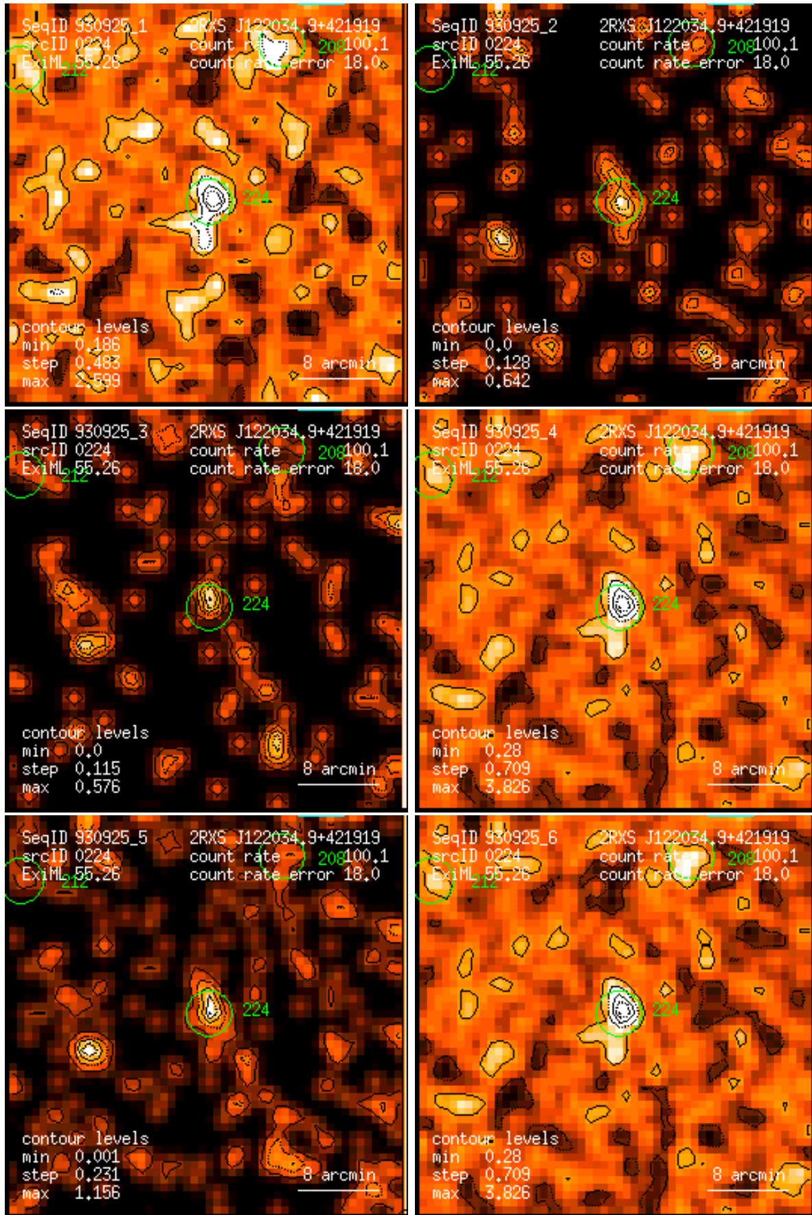
Figure 224: RASS 930925: detection 0224: band rate images, Gaussian filter: (1) PSPC channels 11 – 41, (2) 52 – 90, (3) 91 – 201, (4) 11 – 235, (5) 52 – 201, (6) 11 – 201. Broad band rates in counts/ks. Band rate contour levels in counts/ks/arcmin 2 .
