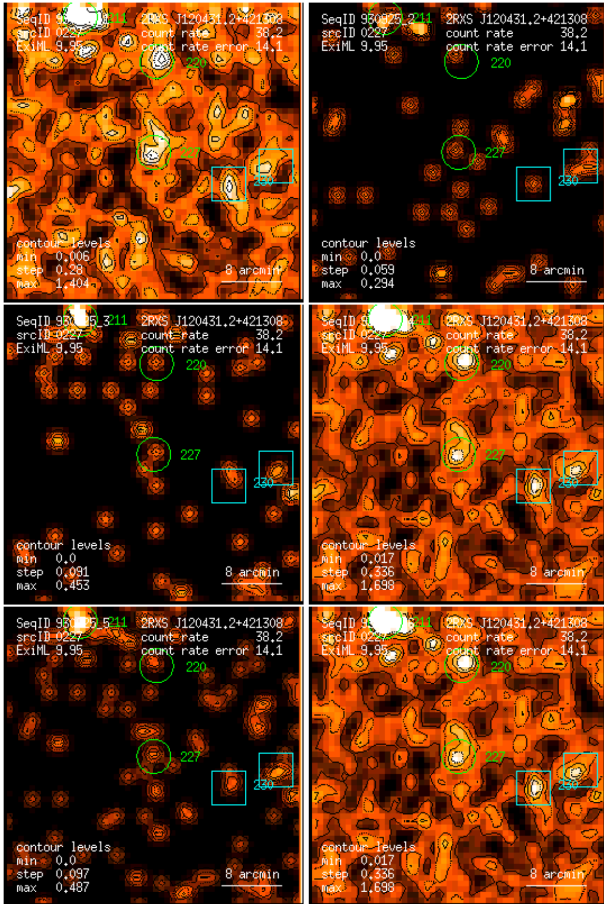
Figure 227: RASS 930925: detection 0227: band rate images, Gaussian filter: (1) PSPC channels 11 – 41, (2) 52 – 90, (3) 91 – 201, (4) 11 – 235, (5) 52 – 201, (6) 11 – 201. Broad band rates in counts/ks. Band rate contour levels in counts/ks/arcmin 2 .
