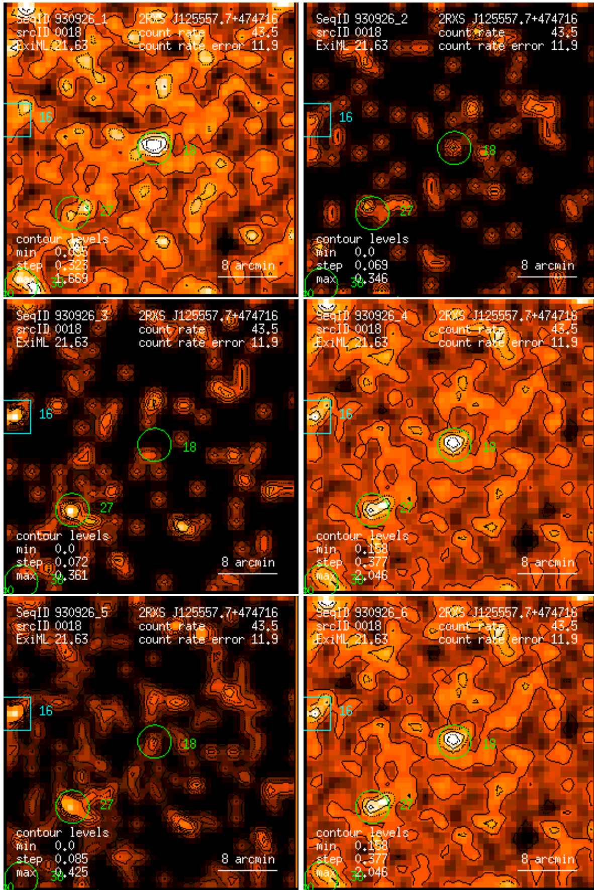
Figure 18: RASS 930926: detection 0018: band rate images, Gaussian filter: (1) PSPC channels 11 – 41, (2) 52 – 90, (3) 91 – 201, (4) 11 – 235, (5) 52 – 201, (6) 11 – 201. Broad band rates in counts/ks. Band rate contour levels in counts/ks/arcmin 2 .
