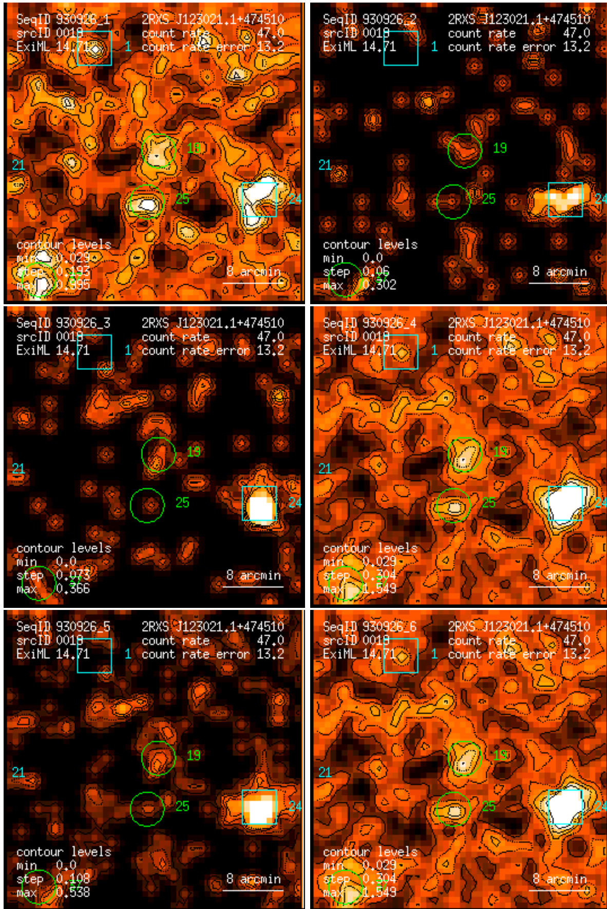
Figure 19: RASS 930926: detection 0019: band rate images, Gaussian filter: (1) PSPC channels 11 – 41, (2) 52 – 90, (3) 91 – 201, (4) 11 – 235, (5) 52 – 201, (6) 11 – 201. Broad band rates in counts/ks. Band rate contour levels in counts/ks/arcmin 2 .
