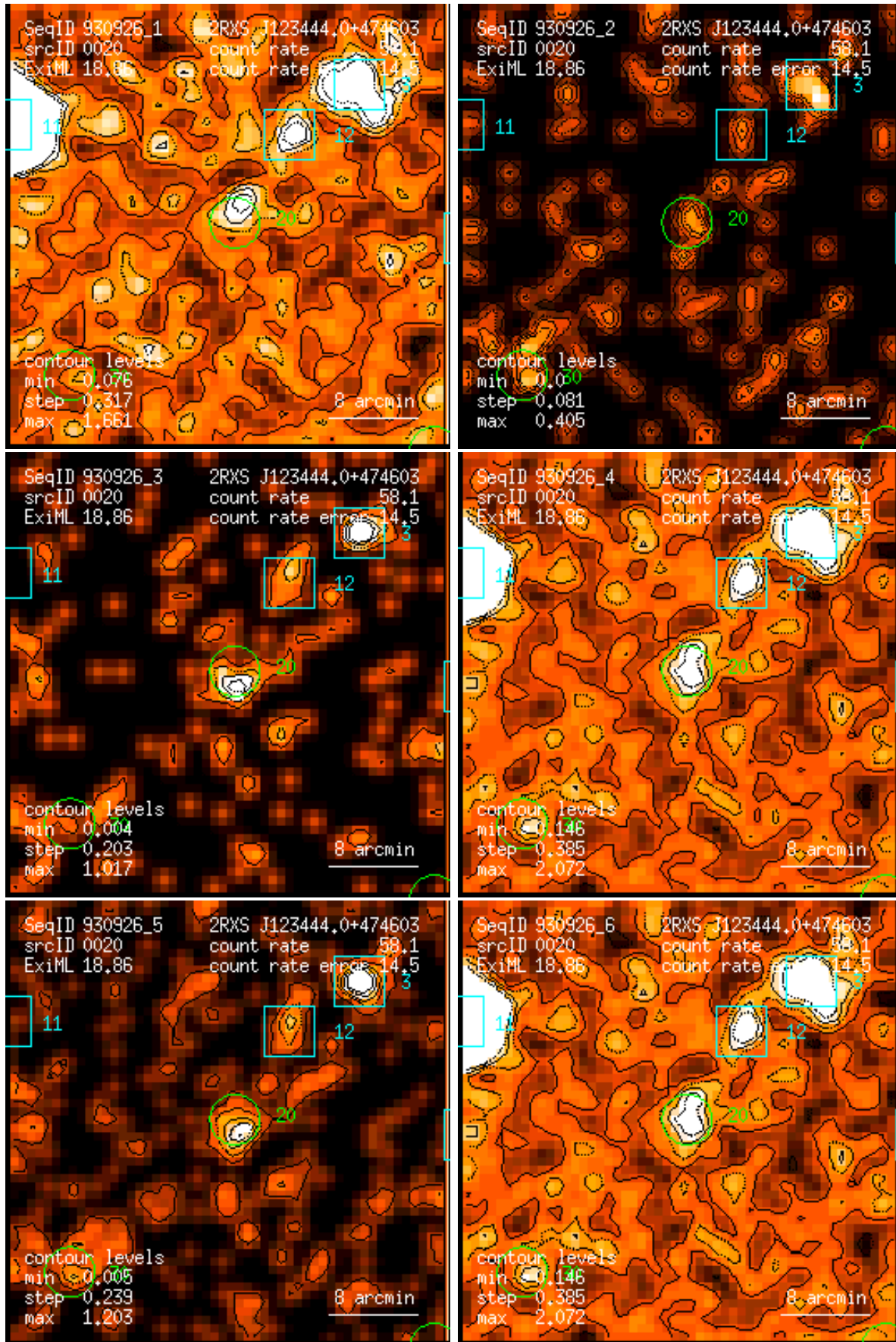
Figure 20: RASS 930926: detection 0020: band rate images, Gaussian filter: (1) PSPC channels 11 – 41, (2) 52 – 90, (3) 91 – 201, (4) 11 – 235, (5) 52 – 201, (6) 11 – 201. Broad band rates in counts/ks. Band rate contour levels in counts/ks/arcmin 2 .
