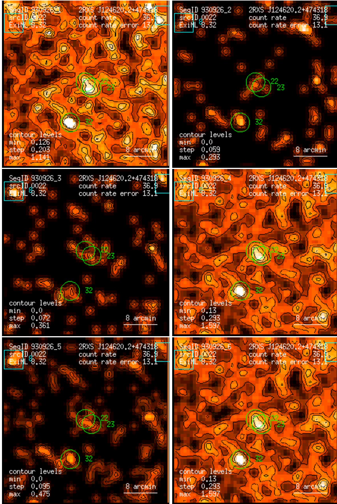
Figure 22: RASS 930926: detection 0022: band rate images, Gaussian filter: (1) PSPC channels 11 – 41, (2) 52 – 90, (3) 91 – 201, (4) 11 – 235, (5) 52 – 201, (6) 11 – 201. Broad band rates in counts/ks. Band rate contour levels in counts/ks/arcmin 2 .
