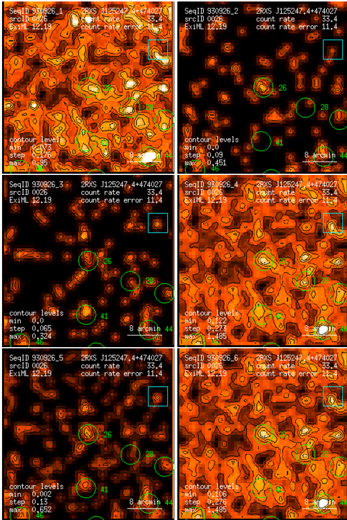
Figure 26: RASS 930926: detection 0026: band rate images, Gaussian filter: (1) PSPC channels 11 – 41, (2) 52 – 90, (3) 91 – 201, (4) 11 – 235, (5) 52 – 201, (6) 11 – 201. Broad band rates in counts/ks. Band rate contour levels in counts/ks/arcmin 2 .
